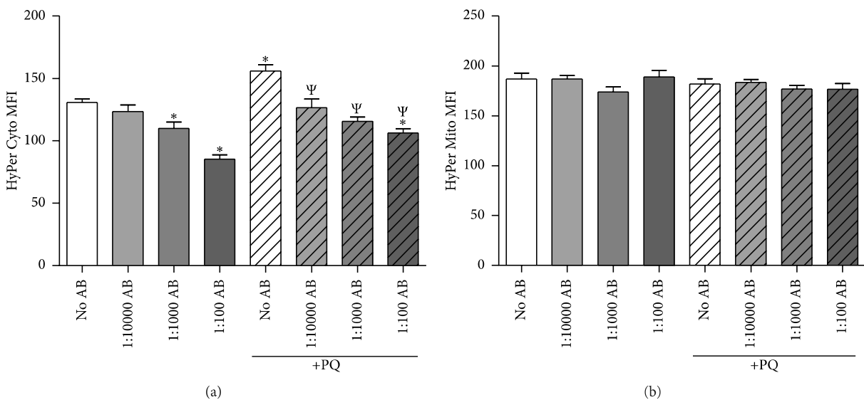
FIGURE 3: AB decreases cellular H 2 O 2 in a dose-dependent fashion. NG108-15 cells were treated with 50 μM PQ with various doses of AB. AB was added 24 hours prior to PQ; cells were analyzed 48 hours after PQ administration. (a) Cytoplasmic H 2 O 2 levels measured by a cytoplasmic-targeted H 2 O 2 -sensitive fluorescent protein (HyPer Cyto). N = 4. (b) Mitochondrial H 2 O 2 levels measured by a mitochondria-targeted H 2 O 2 -sensitive fluorescent protein (HyPer Mito). MFI = mean fluorescence intensity. N = 4. * p < 0.05 versus No AB; Ψ p < 0.05 versus PQ-No AB.
