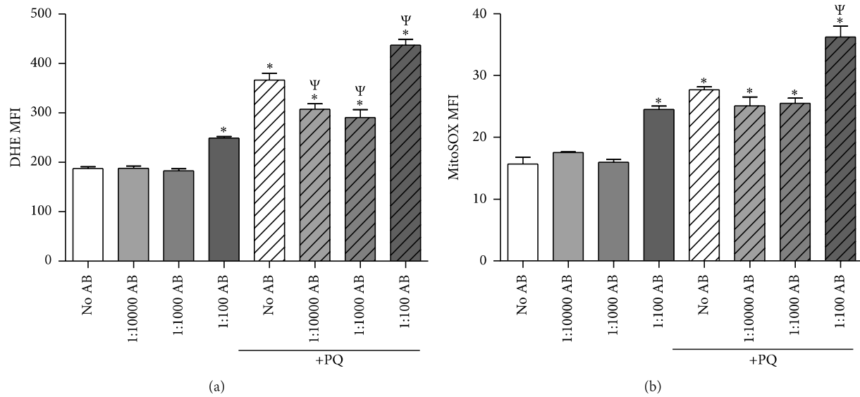
FIGURE 2: Low-dose AB decreases PQ-induced increase in O 2 •- levels. NG108-15 cells were treated with 50 μM PQ with various doses of AB. AB was added 24 hours prior to PQ; cells were analyzed 48 hours after PQ administration. (a) Total cellular O 2 •- levels measured by dihydroethidium (DHE) oxidation and flow cytometry. N = 4. (b) Mitochondrial-specific O 2 •- levels measured by MitoSOX oxidation and flow cytometry. MFI = mean fluorescence intensity. N = 4. * p < 0.05 versus No AB; Ψ p < 0.05 versus PQ-No AB.
