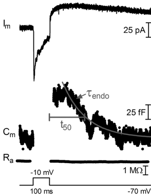
Figure 9: Fast endocytosis in rods.
