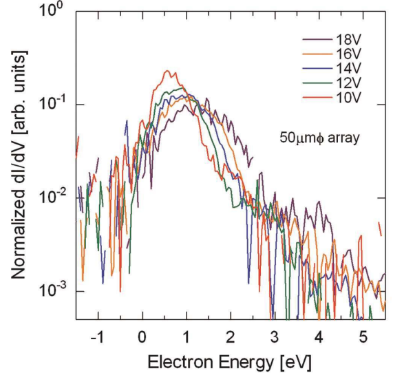
Fig. 5 Energy spectra of emitted electrons from an nc-Si MOS cathode array at various gate voltage.
