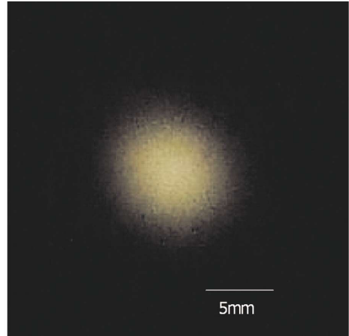
Fig. 6 Emission image from the nc-Si MOS cathode array.
