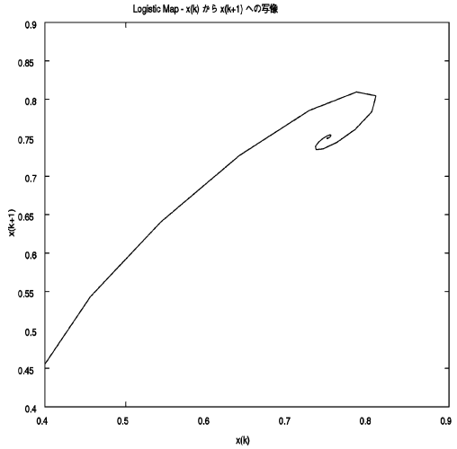
図7 制御過程の写像 x(k) \rightarrow x(k+1) (不動点 x_f=0.75 ) Figure 7 Map x(k) \rightarrow x(k+1) of control process (fixed point x_f=0.75 ).
