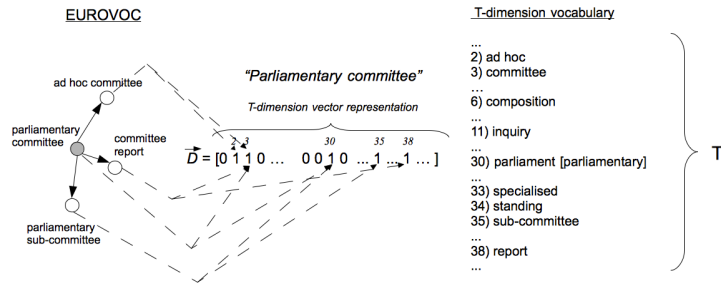
Figure 3. T -dimension vectorial representation of a thesaural concepts \vec{d} .
