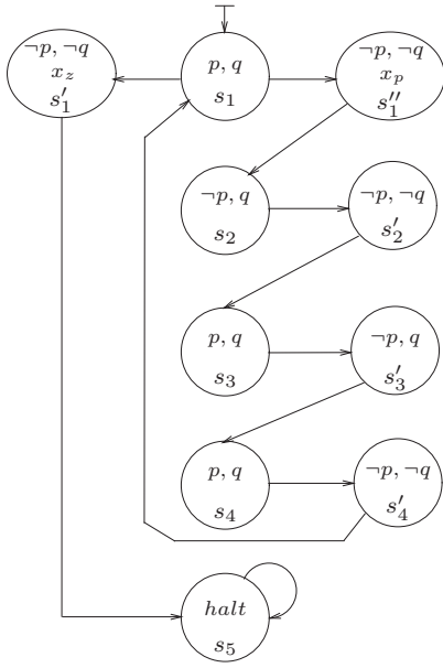
Fig. 4. The Boolean Kripke structure corresponding to the counter machine of Example 8.
