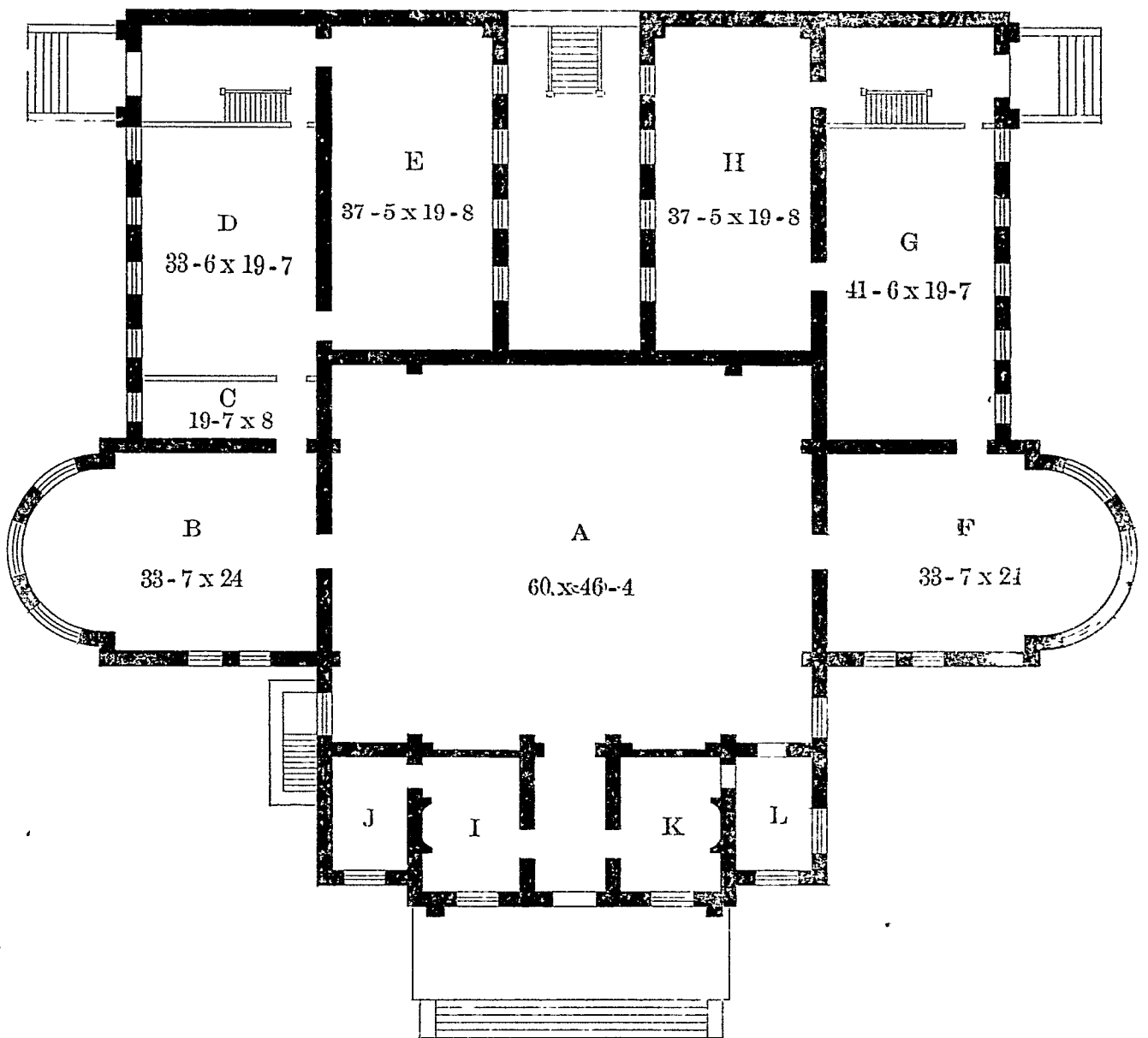
Ground-Plan (Science Hall). 1st Floor.
