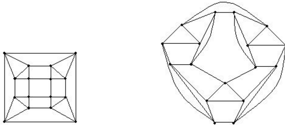
Figure 2.2: A [16,4] -graph and a [17,4] -graph
