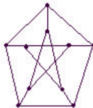
Figure 1.7: The Petersen Graph
