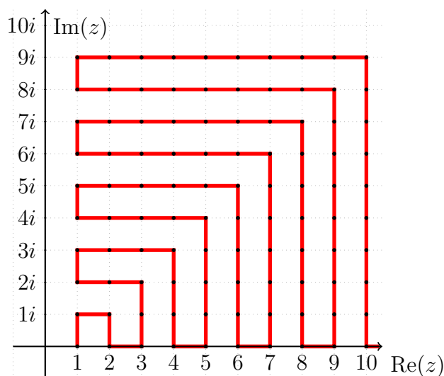
Figure 2: Spiral Ordering of Gaussian Integers
