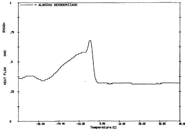
Figure 4 DSC melting curve for deodorized cottonseed oil
