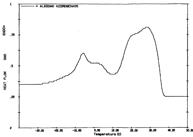
Figure 5 DSC melting curve for hydrogenated cottonseed oil
