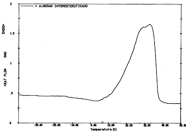
Figure 6 DSC melting curve for interesterified cottonseed oil
