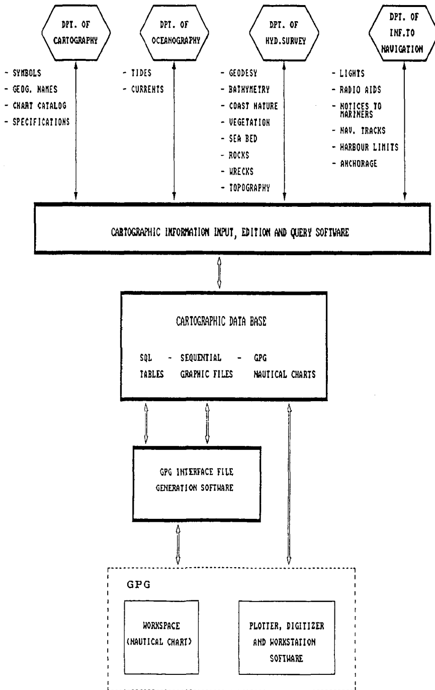
FIG. 2.- 'AUTOCARTA' System Development.
