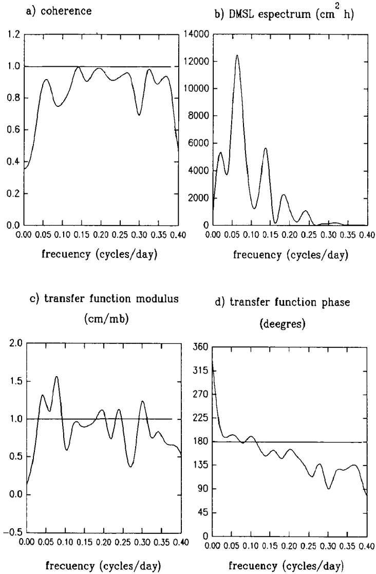
FIG. 3.- Results from cross spectral analysis between atmospheric pressure in San Fernando and MSL in Cádiz. Atmospheric pressure (mb) as the input and MSL (cm) as the output.
