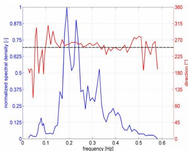
Figure 7: First results from the radar gauge array. The normalized spectral density (blue) and the direction of the waves (red) are illustrated as functions of frequency. The black dotted line denotes the mean wind direction.
