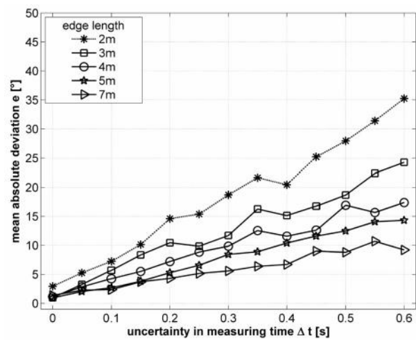
Figure 5: Resolving power of the radar gauge array, determined by adopting simulated computer data. The mean absolute deviation of the estimated direction is shown for Gaussian-distributed time lags with standard deviations up to 0.6 s. Additionally, the dependence on the edge length can be examined.
