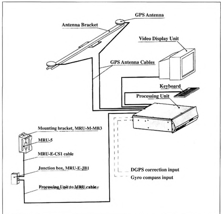
Figure 3: Kongsberg Seatex Seapath 200
