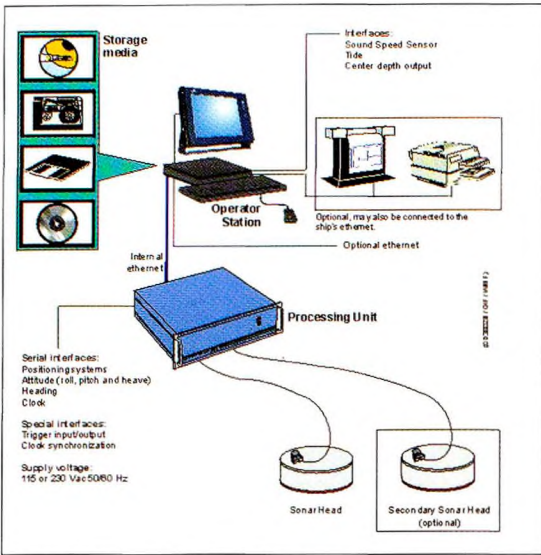
Figure 2: Kongsberg Simrad EM 3000 multi beam echo sounder
