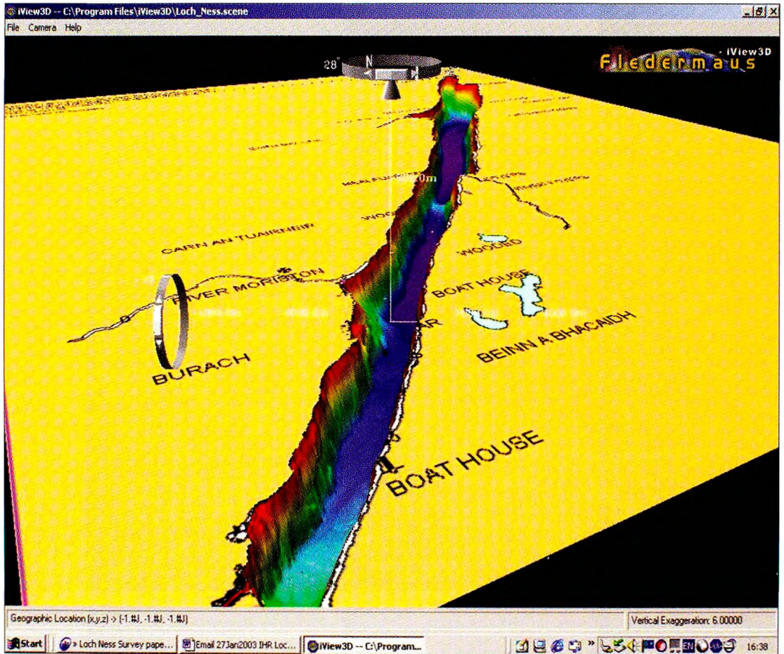
Figure 4: Loch Ness bathymetry visualised in Fledermaus. A, B, C: Objects found in northern part in the imagery data
