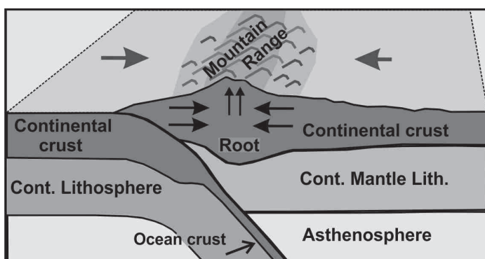
Figure 3. Model of continental collision and crustal thickening for mountain-belt formation. For the Cordillera there is no crustal root, so this is not a valid model for the high elevation.
