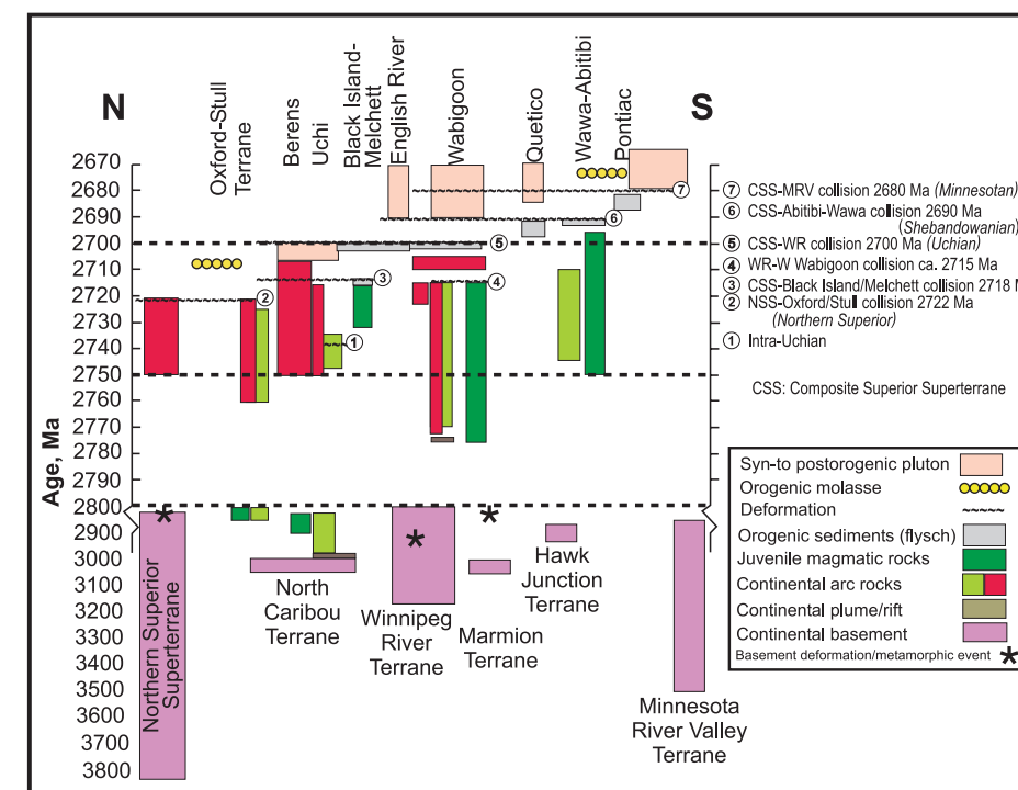
Figure 11 Cladogram (cf. Hoffman, 1989) illustrating timing of assembly of the Superior Province from continental and oceanic fragments. Note successive merging of terranes between 2720 and 2680 Ma.
