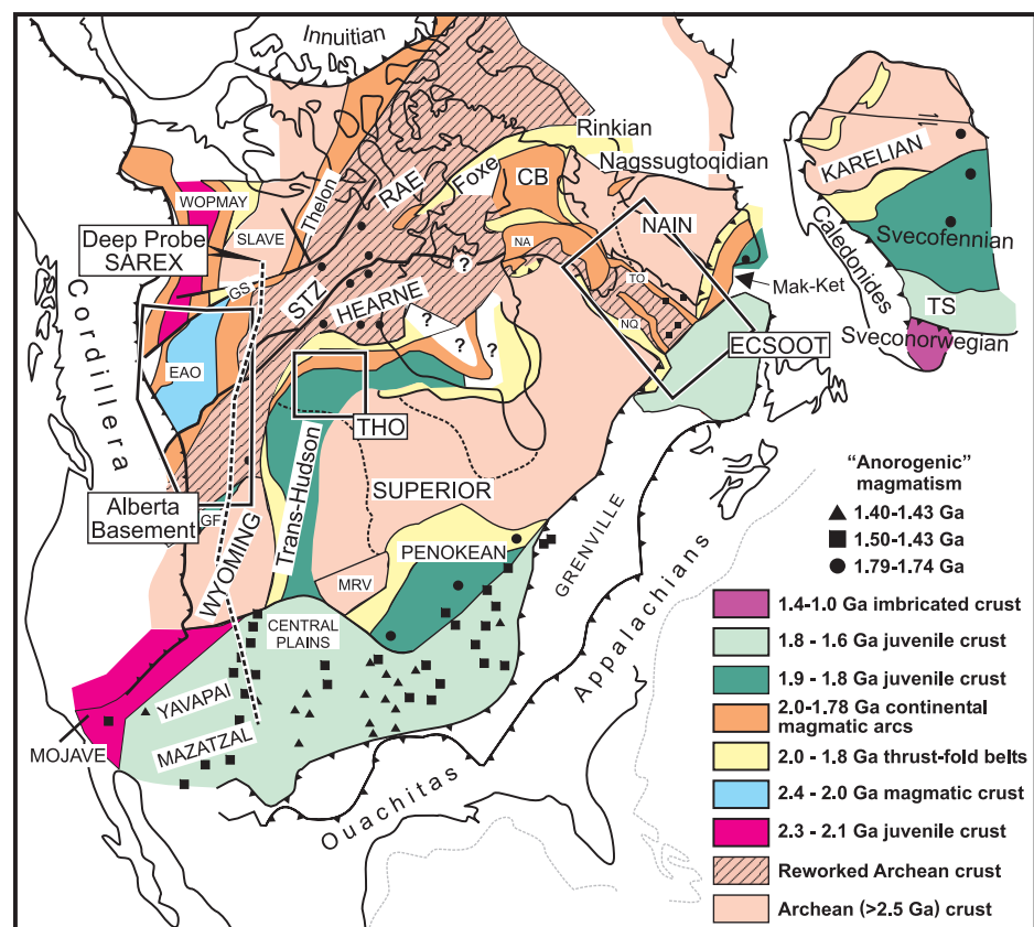
Figure 8 Paleoproterozoic tectonic elements of North America (modified after Hoffman, 1989). CB: Cumberland batholith; GF: Great Falls Tectonic Zone; GS: Great Slave Lake shear zone; NA: Narsajuaq arc; NQ: New Quebec orogen; STZ: Snowbird Tectonic zone; TO: Torngat orogen.
