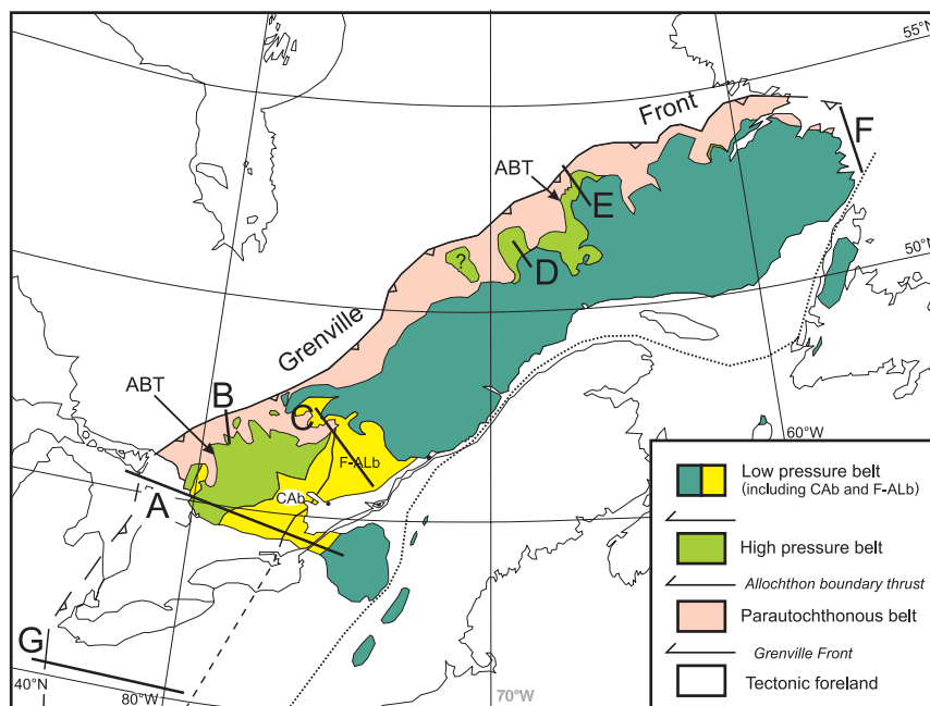
Figure 6 Sketch map of the Grenville Province showing the distribution of orogen-scale belts (after Rivers et al., 2002). Thick lines labeled A to G are the locations of seismic transects. ABT: Allocthon boundary thrust; CAB: Composite Arc belt; F-ALb: Frontenac-Adirondack Lowland belt.
