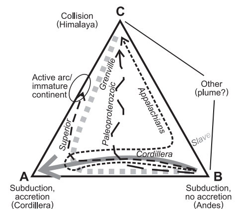
Figure 14 Orogenic classification diagram developed at the workshop to describe the development of orogens in terms of subduction, accretion and collision. Additional end-members may be necessary in some orogens to describe non-plate tectonic processes.
