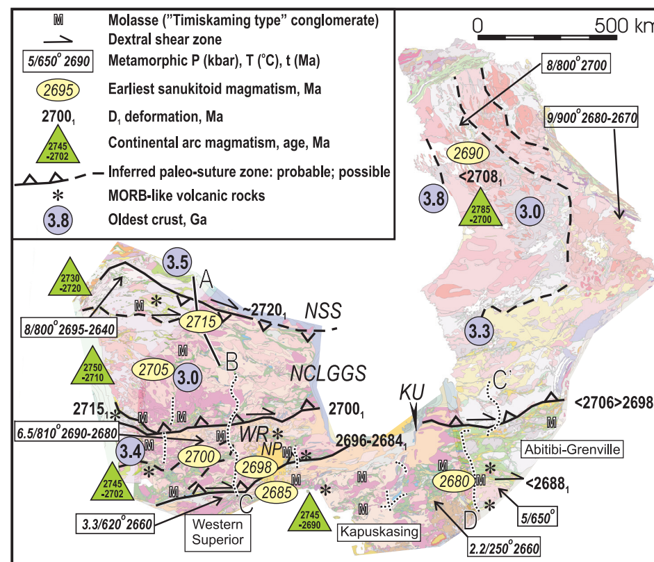
Figure 10 Tectonic elements of the Superior Province, showing old cratons and other features: NSS: Northern Superior superterrane; NCLGGS: North Caribou- La Grande- Goudalie superterrane; WR: Winnipeg River terrane; KU: Kapuskasing uplift; NP: Nipigon plate. Features of tectonic significance are indicated in the legend. A, B, C, C', D indicate segments of cross-section in Figure 9.
