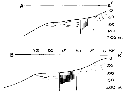
Fig. 1 (a) Diagram showing geomorphic zonation of a beach to inner shelf profile. (b) Plan and sectional views of two modern inner shelf areas, the low-energy Atlantic coast and the high-energy, wave-dominated Oregon coast.
