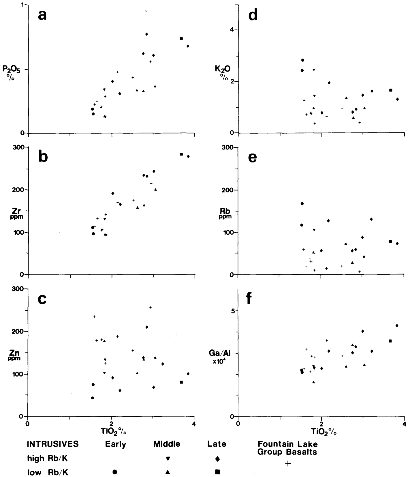
Fig. 6. Plots of selected elements against \text{TiO}_2 (a proxy for degree of fractionation) for the mafic rocks of the North River pluton. Shown for comparison are Fountain Lake basalts. (a) \text{P}_2\text{O}_5 ; (b) Zr; (c) Zn; (d) \text{K}_2\text{O} ; (e) Rb; (f) \text{Ga}/\text{Al} .
