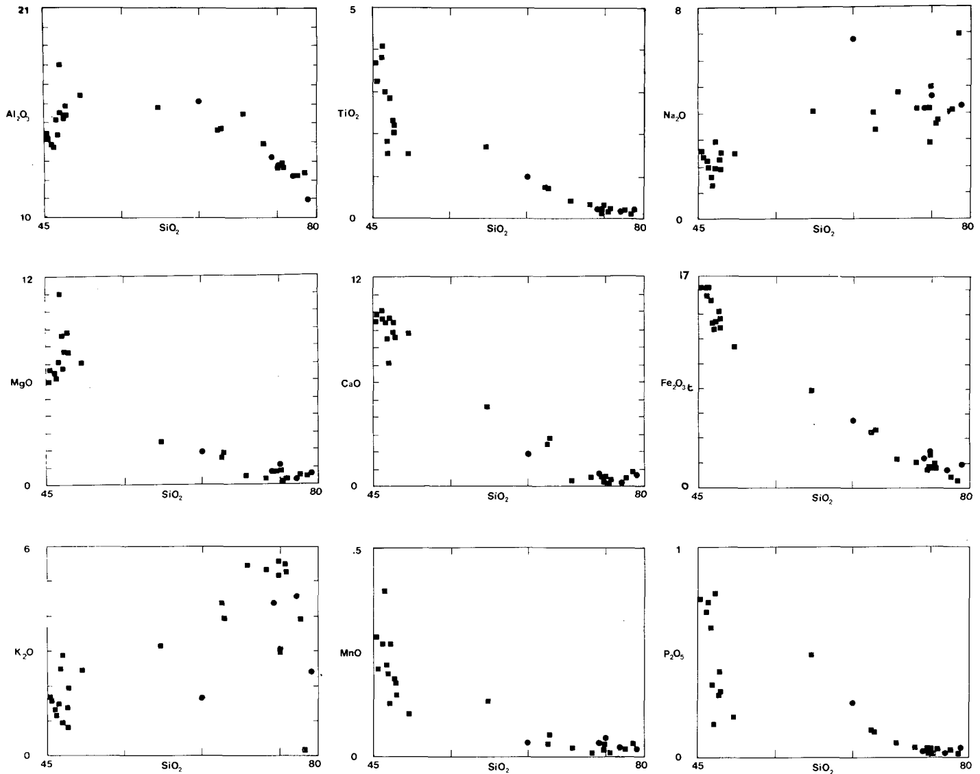
Fig. 3. Major element oxides plotted against \text{SiO}_2 for rocks of the the North River pluton and adjacent hypabyssal rocks. Solid squares - North River pluton rocks; solid circles - hypabyssal rocks from the western margin of the pluton. Samples with between 55% and 70% \text{SiO}_2 are from rocks with hybrid texture. Analyses recalculated on a volatile-free basis.
