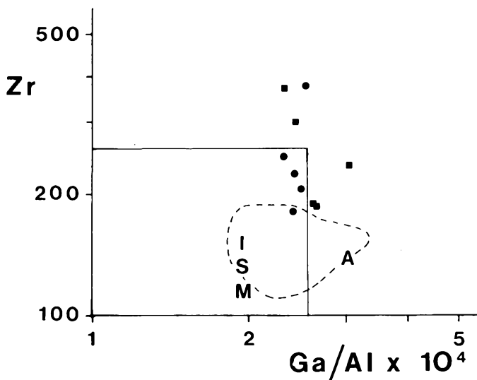
Fig. 5. Plot of Zr against Ga/Al for felsic plutonic rocks (squares) and microgranite dykes (circles). Rectangular box separates A-type granites (upper right) from I, S and M-type granites (after Whalen et al. , 1987). Dashed line shows limit for the Ackley pluton I-type granites (Tuach et al. , 1986).
