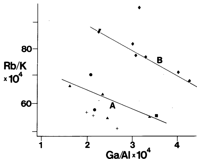
Fig. 7. Plots of Rb/K v. Ga/Al for the mafic rocks of the North River pluton, showing the recognition of assemblages with low and high Rb/K ratio (c.f. Table 1). Symbols as in Figure 6.
