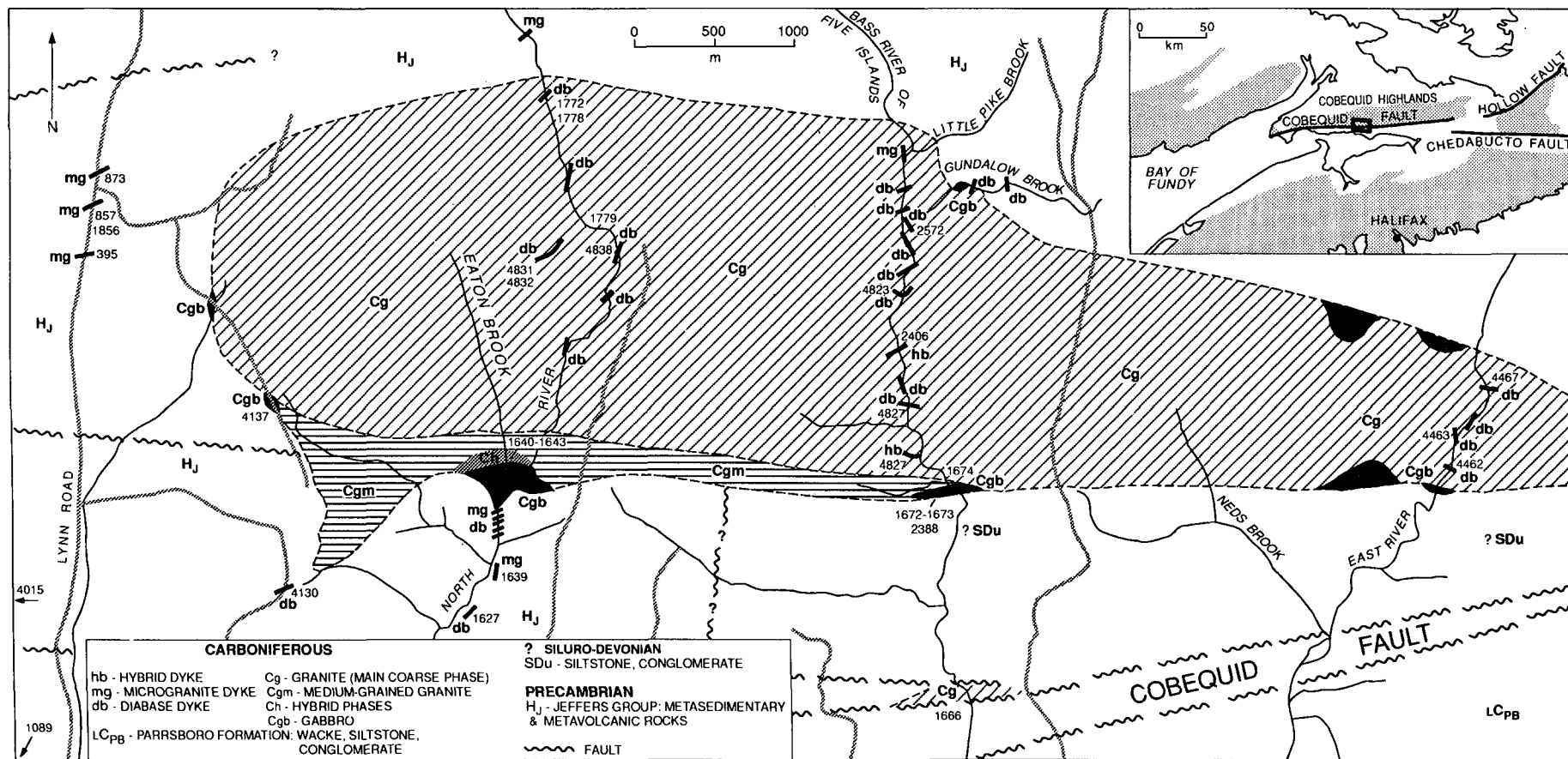
Fig. 2. Geological map of the North River pluton showing location of analysed samples.
