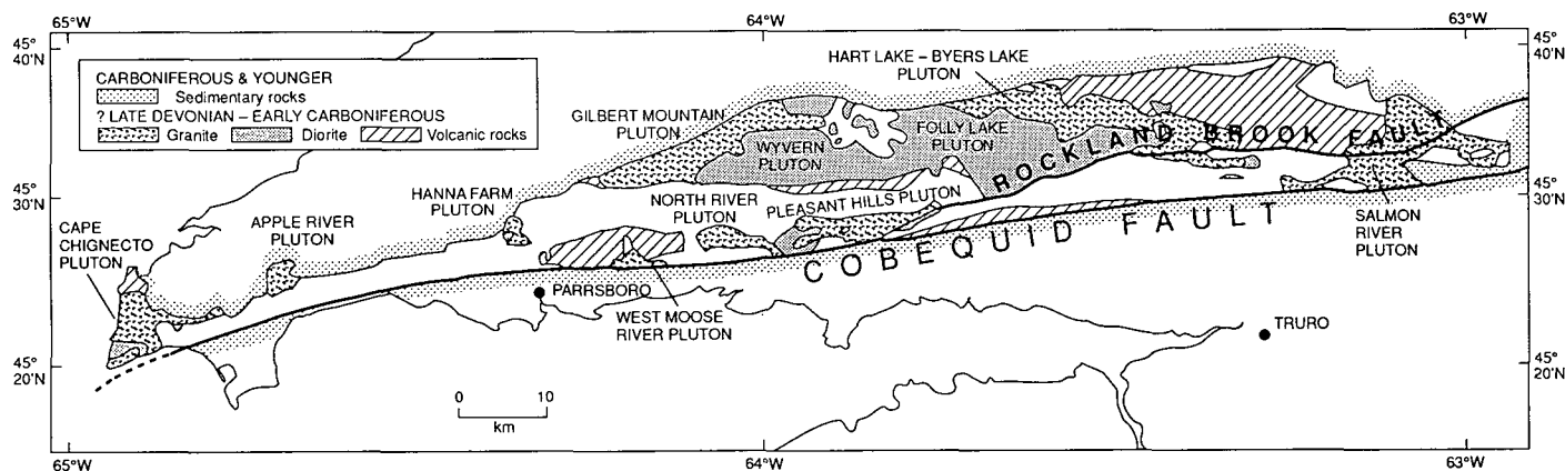
Fig. 1. Regional map of the Cobequid Highlands showing location of the North River pluton. Based on Murphy et al. (1988), Pe-Piper and Turner (1988) and Waldron et al. (1989).
