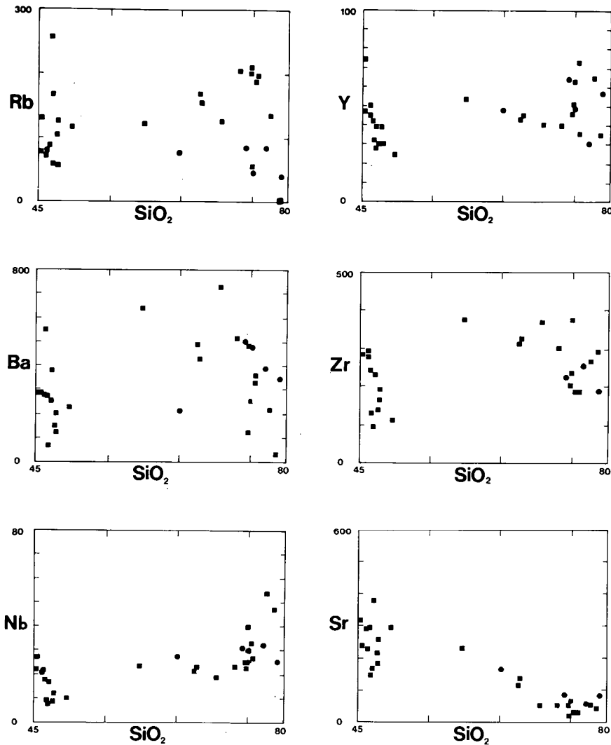
Fig. 4. Variation in selected trace elements within the North River pluton and adjacent hypabyssal rocks. Symbols as in Figure 3.
