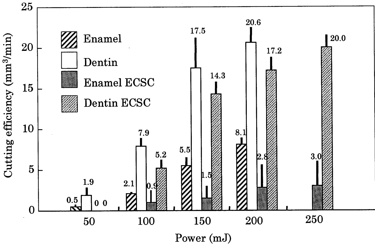
Fig. 4 Cutting efficiency
