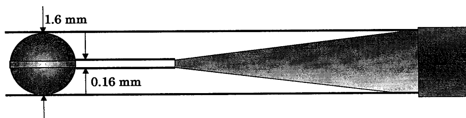
Fig. 1 Shape of contact tip
