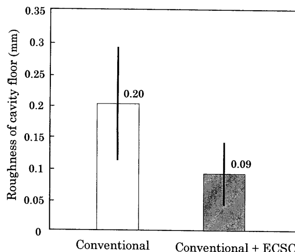
Fig. 7 Roughness of cavity floor
