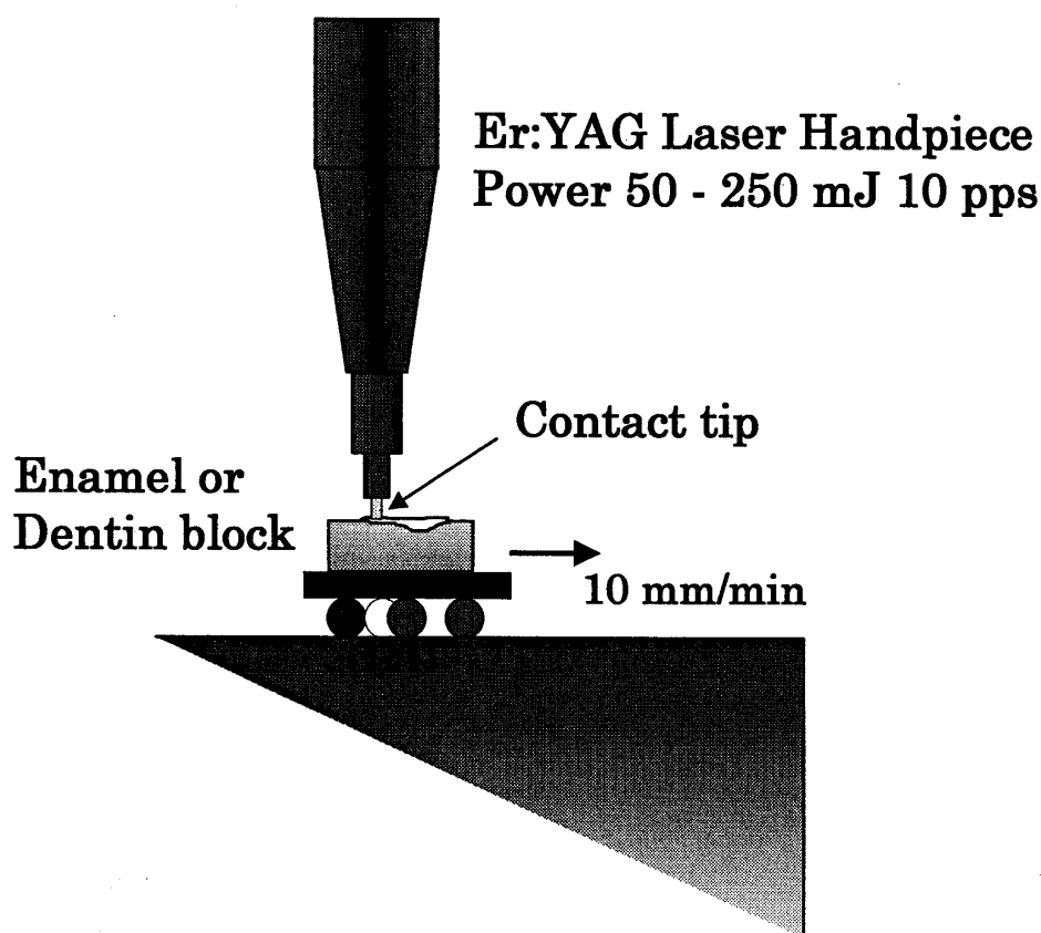
Fig. 2 Test method for cutting efficiency evaluation Taper angle of cavity : (a+a')/2 Roughness of cavity floor : b
