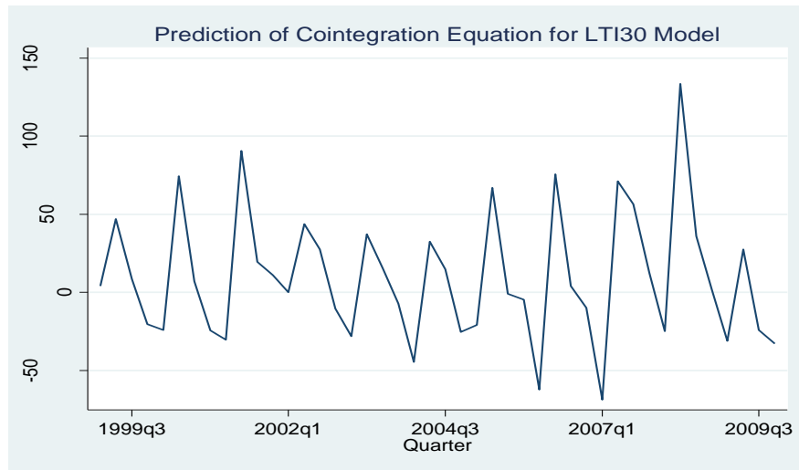
Figure 1: Line graph for cointegration equation of the LTI Model from 1999 to 2009
