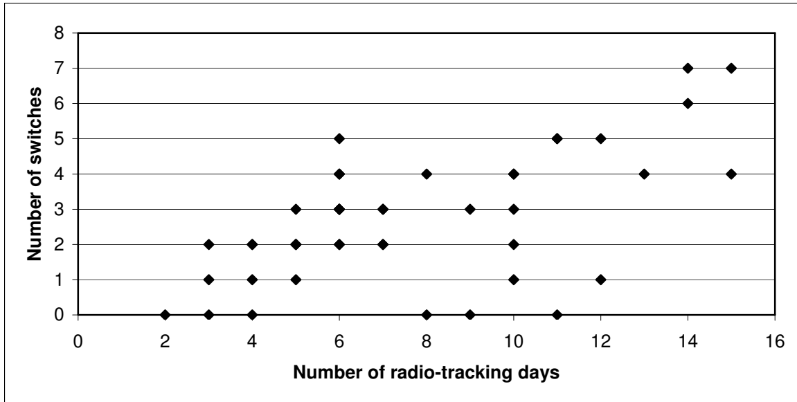
Figure 1.10. Relationship between number of switches and number of days that a bat was radio tracked ( n = 45 ; r = 0.59 ; P < 0.001 ).
