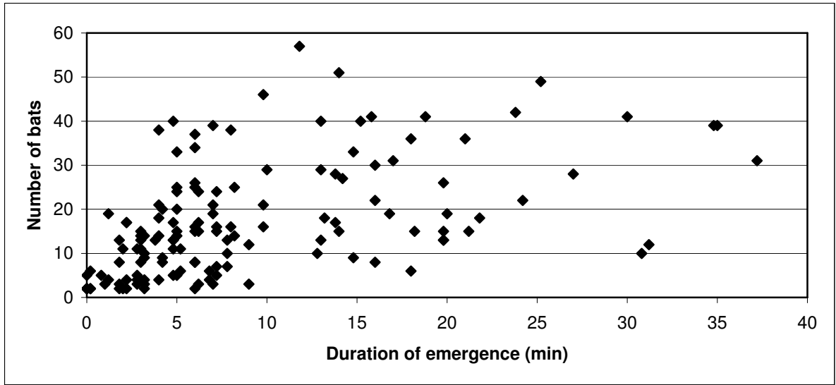
Figure 1.6. Relationship between number of bats and length of time (min) for all bats to exit the roost ( n = 136 ; r = 0.51 ; P < 0.001 ). Only observations of \geq 2 bats are included.
