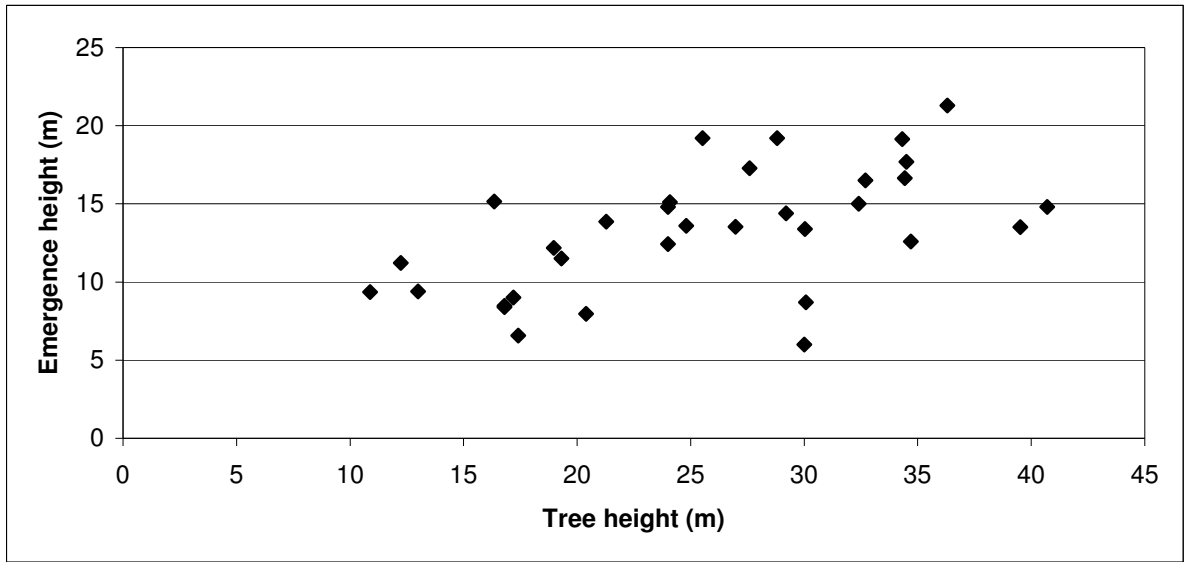
Figure 1.12. Relationship between the height of the emergence site and height of the tree ( n = 33 ; r = 0.56 ; P = 0.001 ).
