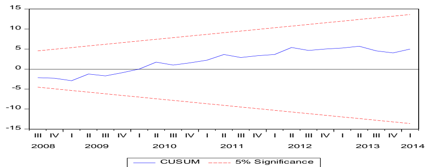
Figure 2. Result of CUSUM Test for Stability of the Government Expenditure Model
