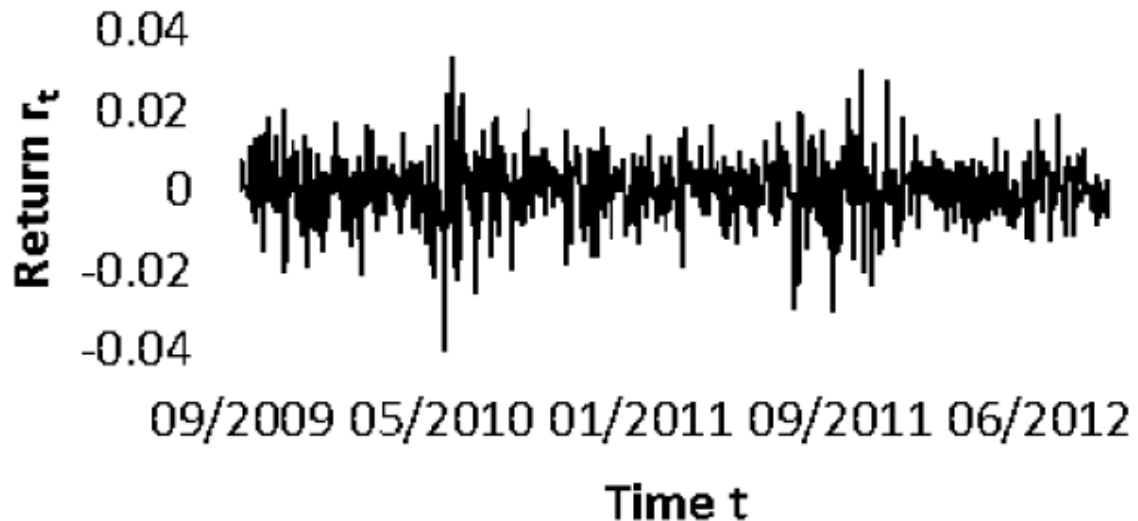
Figure 1. Time Series Plot Continuous Returns
