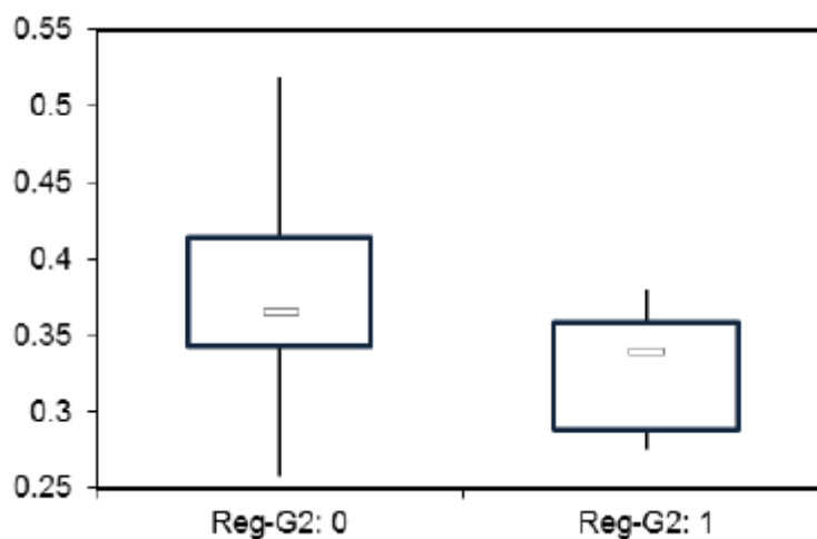
Figure 4. Manual MLR Including Constant
