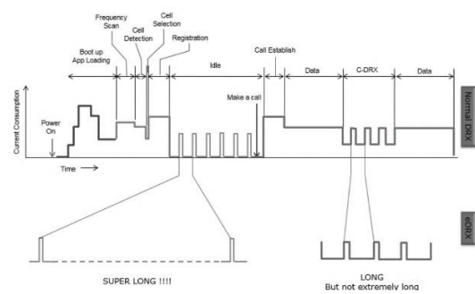
Figure 6, eDRX vs. DRX mechanism
