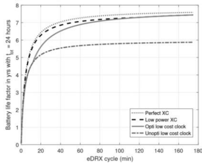
Figure 7, battery life time under different eDRX values Fig. 8: Battery life time for under different scenarios
