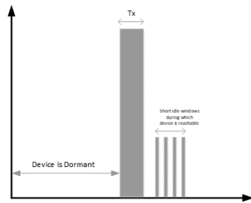
Figure 3, PSM operation
