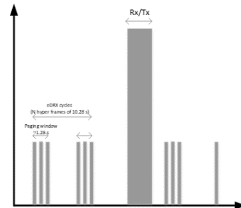
Figure 4, eDRX operation
