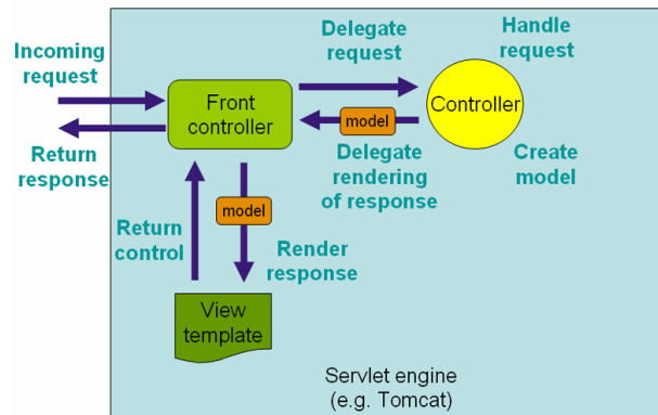
Figure 28: Dispatcher Servlet
