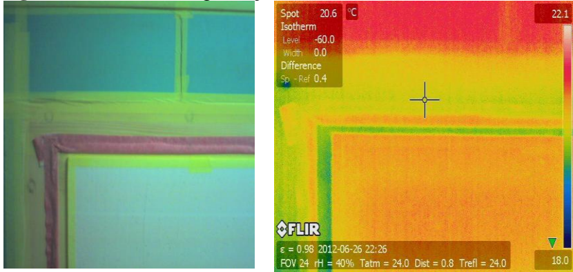
Figure 5: Thermal image of joint sealed with classical PU foam shows heat losses
