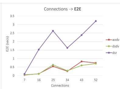
Fig. 8. E2E vs. Number of Connections
