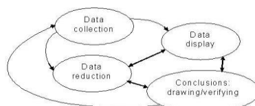
Figure 1: Component of Data Analysis: Interactive Model by Miles and Huberman (1994: 12)
