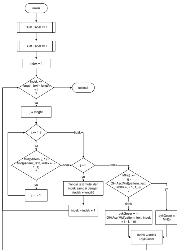
Gambar. 2. Flowchart Algoritma Boyer-moore
