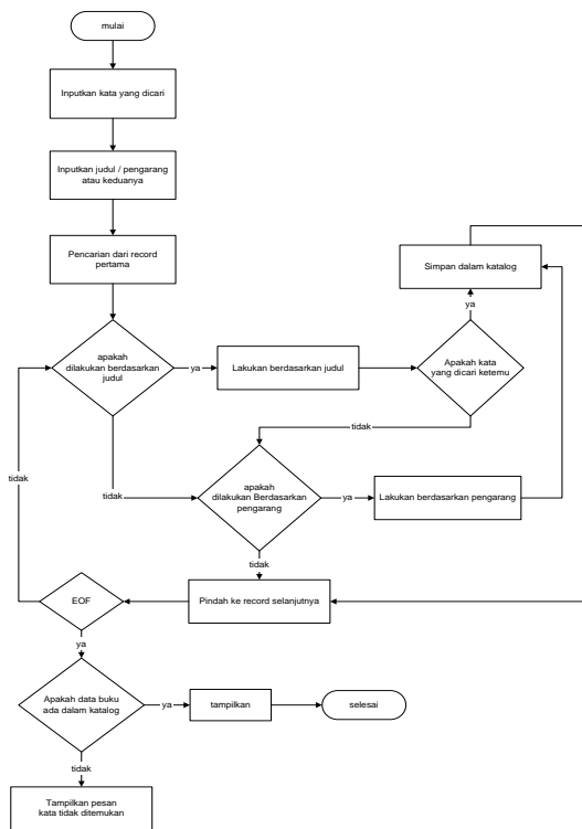
Gambar 3. Flowchart sistem
