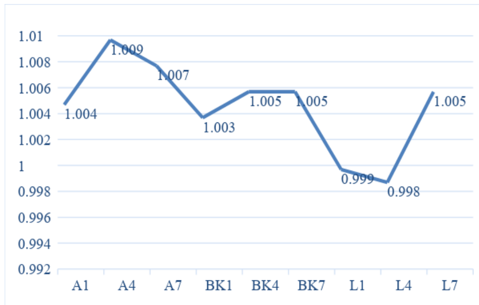
Graph 5: Specific Gravity of Soil Samples
