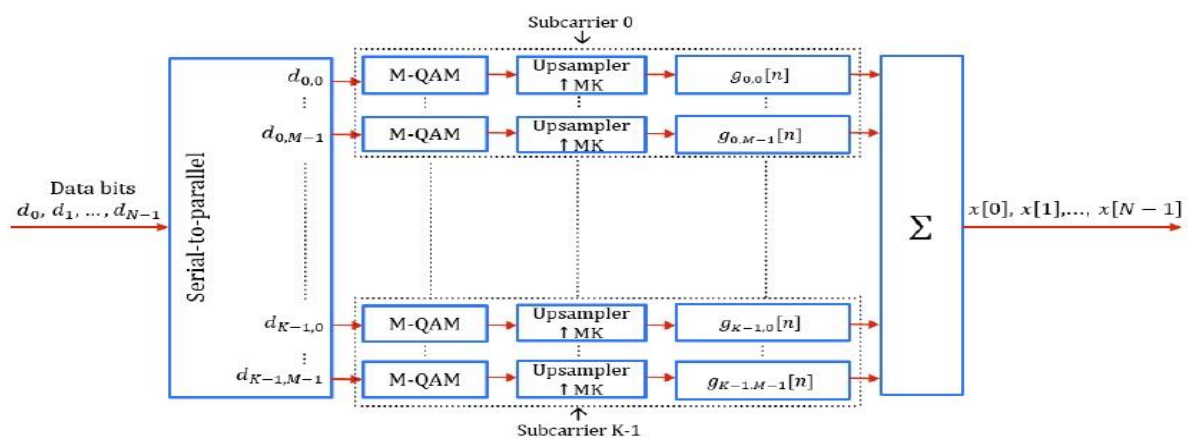
Figure 4. Modulator of GFDM as block diagram.
