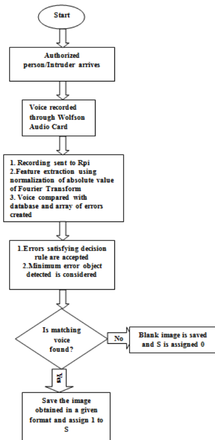
Figure 4: Flowchart for Speech Recognition Sub-system
