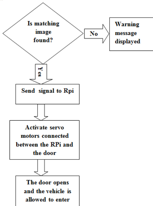
Figure 2: Flowchart for Automatic Number Plate Recognition Sub-system
