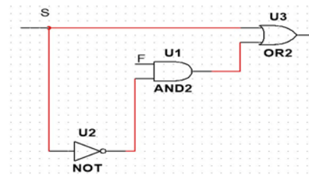
Figure 5: Circuit Diagram of overall system
