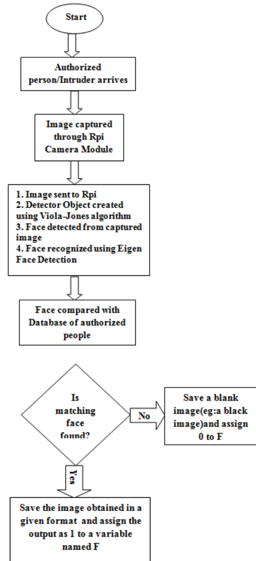
Figure 3: Flowchart for Face Detection and Recognition Sub-System
