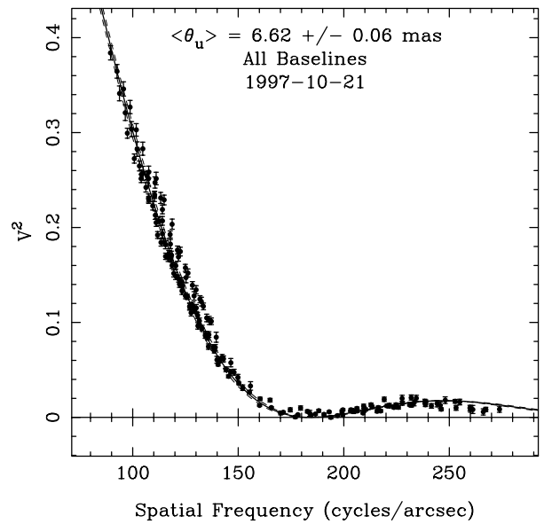
FIG. 1.—Plot of calibrated V^2 vs. spatial frequency for seven scans of \gamma Aql shown with a simple uniform disk fitted to the data. The best fit to the data (solid line) is \langle \theta_u \rangle = 6.62 \pm 0.06 mas (with the dashed lines representing the error of the mean).
