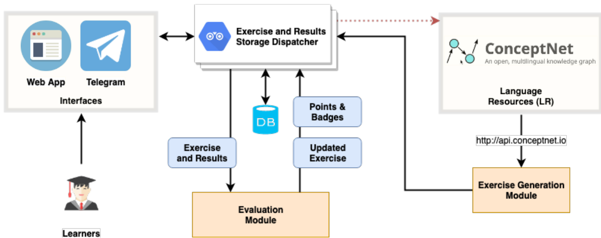
Figure 1: An overview of the vocabulary trainer architecture, depicting the main modules of the architecture, the data interchange between them and user interaction at the interface level.
