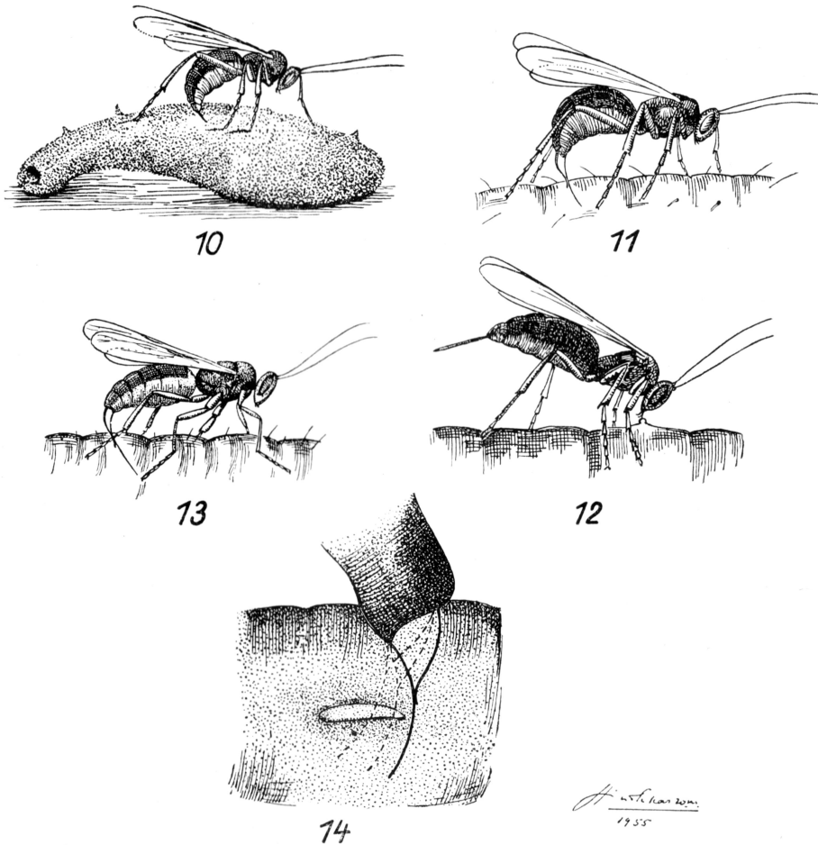
Fig. 10—14. Oviposition and feeding habits of Microbracon gelechia Ashm. Fig. 10. Female ovipositing through the cocoon of the host. — Fig. 11. Female stabbing a naked larva prior to oviposition. — Fig. 12. Female feeding through the puncture of host larvae as a result of stabbing. — Fig. 13. Female in the act of oviposition on Corcyra larva. — Fig. 14. Close up of the ovipositing abdomen of the female
