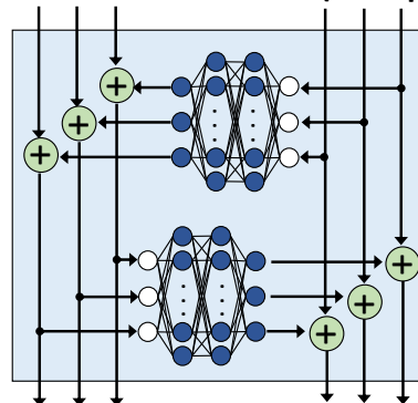
Figure 1. Boltzmann Generators. a) A Boltzmann Generator is trained by minimizing the difference between its generated distribution and the desired Boltzmann distribution. It is used by transforming samples from a simple (e.g., Gaussian) distribution to generated configurations. To compute thermodynamics, such as configurational free energies, the samples must be reweighted to the Boltzmann distribution. b) The Boltzmann Generator is composed of invertible neural network blocks. Here, a volume-preserving block is shown as an example.
