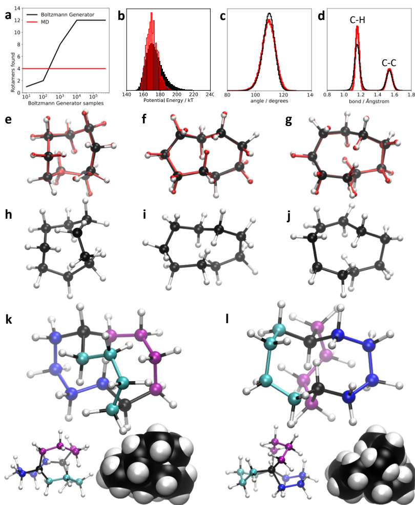
Figure 4. Exploration of new states and direct sampling of cyclical molecule structures: Cyclononane C_9H_{18} (a-j) and bicyclo[4.4.4]tetradecane C_{14}H_{26} (k-l). a) Number of distinct rotamers sampled with Boltzmann Generator that is initialized with MD data containing 4 rotamer states. b) Potential energy distribution. c-d) Generated bond length and angle distribution compared to MD data. e-g) Boltzmann-generated structures (black) and the most similar structures from replica-exchange MD (red). h-j) Boltzmann-generated structures that are not contained in the MD simulations. k-l) Boltzmann-generated structures of bicyclo[4.4.4]tetradecane C_{14}H_{26} – side-view is shown in large, top view below as ball+stick and space-filling representation. The three chains are colored for better visibility, the connecting carbons are kept dark.
