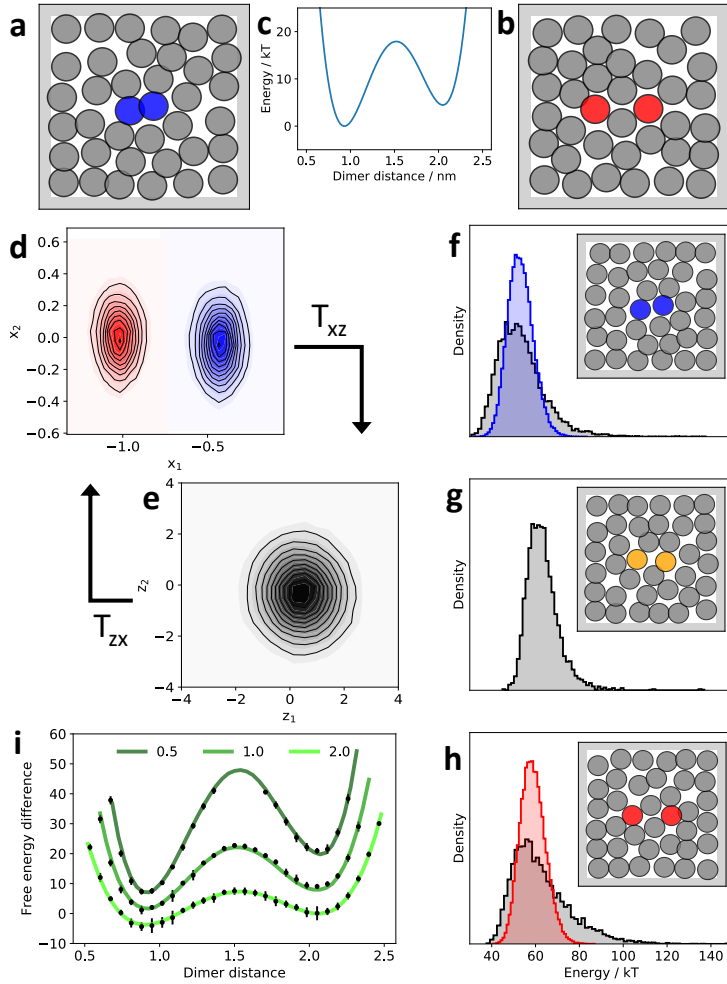
Figure 3. Repulsive particle System with bistable dimer. a,b) Closed (blue) and open (red) configurations from MD simulations (input data). c) Bistable dimer potential. d) Distribution of MD simulation data on x_1, x_2 . e) Distribution of MD simulation data in latent space coordinates z_1, z_2 after training Boltzmann Generator. f, g, h) Potential energy distribution from MD (colored) and Boltzmann generator (grey) for closed (f), open (h) and transition configurations (g). Insets show directly generated samples from Boltzmann Generator. i) Free energy differences as a function of dimer distance and relative temperature sampled with Boltzmann generators (generation and reweighting, bullets with error bars indicating one standard deviation) and umbrella sampling (green lines).
