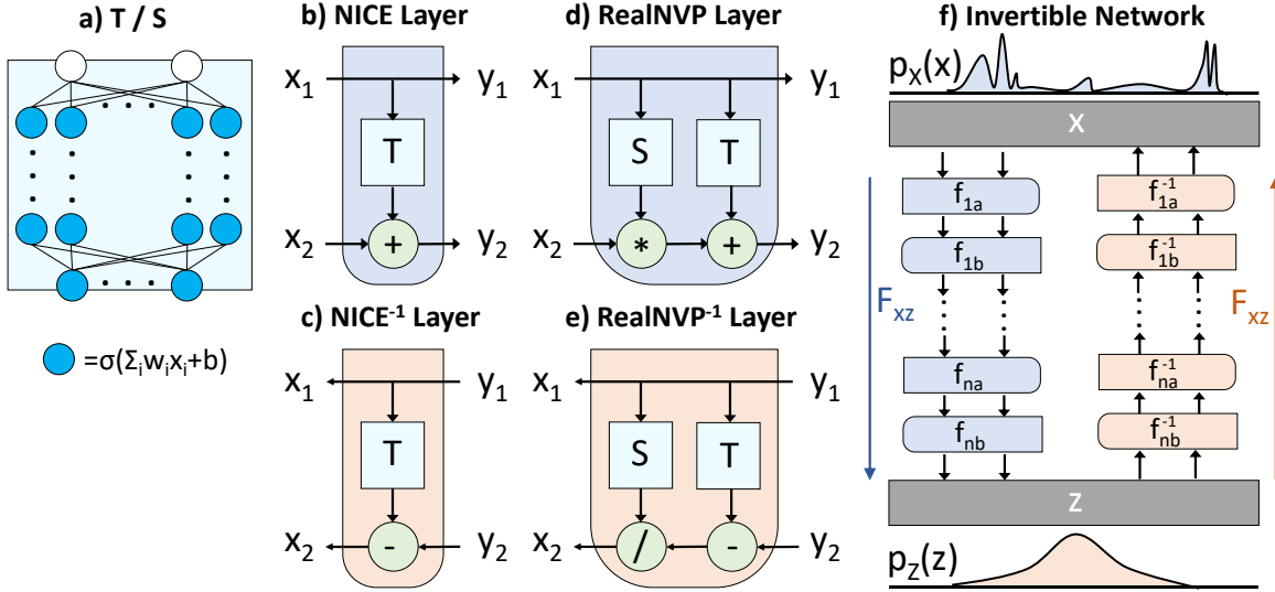
Supplementary Figure 1. Boltzmann Generator network architecture. a) Nonlinear transformations T and S are built with multilayer neural networks. b,c) Volume-preserving NICE layer and its inverse. d,e) Non-volume-preserving RealNVP layer and its inverse. f) Stacking any sequence of these layers with channels exchanges produces the full Boltzmann Generator, and invertible network.
