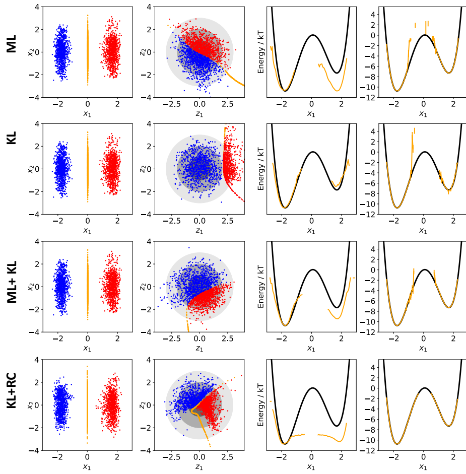
Supplementary Figure 3. Same as Suppl. Fig. 2 but for Boltzmann Generators using RealNVP layers.
