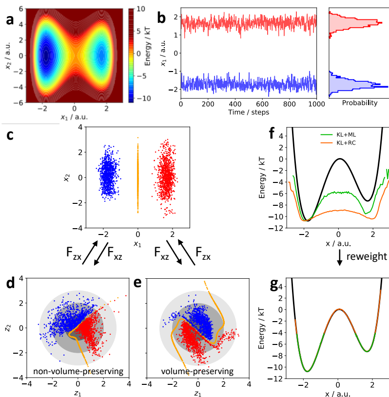
Figure 2. Illustration of Boltzmann Generators for two-dimensional bistable system. a) Two-dimensional potential, x_1 is the slow coordinate. b) Two short simulation trajectories that stay in their metastable states without crossing. c) Distribution of trajectories of b) in configuration space (x_1, x_2) . Transition state ensemble is shown (orange) but not used for training. d,e) Latent-space distribution of trajectories of b) when mapped through trained F_{xz} using transformations that are (d) non-volume preserving and (e) volume-preserving with one global scaling factor. f) Free energy corresponding to distribution sampled by Boltzmann Generators trained by energy and by example (KL+ML, green) and using reaction coordinate training (KL+RC, orange). g) Free energy estimates after reweighting, colors as in (f) .
