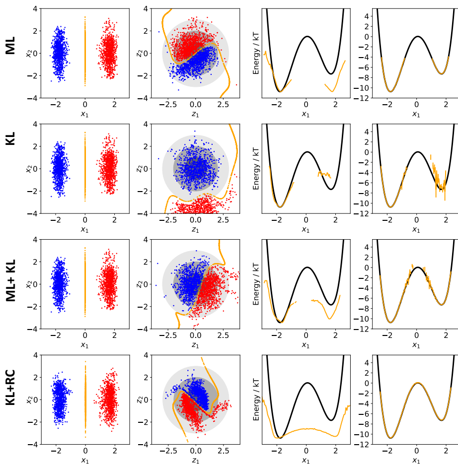
Supplementary Figure 2. Different methods for training Boltzmann Generators with NICE layers using the double well example shown in Fig. 2. Columns show: (1) distribution in configuration space \mathbf{x} , (2) distribution in latent space \mathbf{z} , (3) free energy of Boltzmann Generator output p_X(\mathbf{x}) along x_1 , (4) free energy after reweighting, vertical vars show uncertainties (one standard deviation, 68% percentile). Training uses 200 epochs of ML and then 500 epochs of the method given in the rows, using equal weights for these modes. Training by example (ML) only reproduces the distribution of the training data, which can be reweighted to the Boltzmann distribution in this low-dimensional example but reweighting from the ML-generated distribution fails for high-dimensional examples. Training by energy (KL) alone tends to collapse to a single metastable state. ML+KL combined samples closer to the Boltzmann distribution than ML and avoids metastable state collapse, but samples high-energy transition states with low probability. KL+RC performs best in this example.
