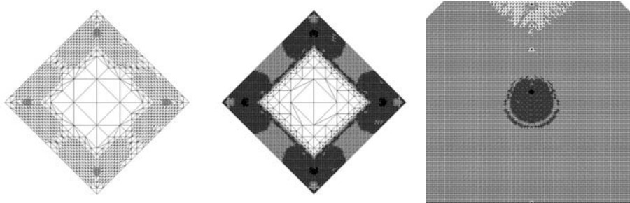
FIGURE 4. Adaptively refined triangulations \mathcal{T}_6 , \mathcal{T}_9 and a zoom into the upper corner of \mathcal{T}_{12} .
