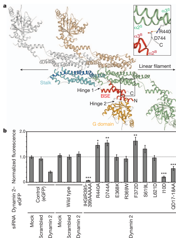
Figure 3 | Stalk interactions with the BSE and PH domain. a , Top view of the dynamin 1 oligomer. The PH domains are not drawn for clarity. The insert shows a close view of the intermolecular BSE–stalk interaction. b , HeLa cells depleted of endogenous dynamin 2 by short interfering RNA (siRNA) were transfected with a plasmid encoding siRNA-resistant dynamin 2–eGFP and allowed to endocytose fluorescently labelled transferrin. In transfected cells, fluorescence was quantified and normalized to mock-treated cells expressing eGFP. Data shown represent mean \pm standard error, * P < 0.05 ; ** P < 0.01 ; *** P < 0.0001 for wild-type versus mutant dynamin 2–eGFP, as determined by t -test.
