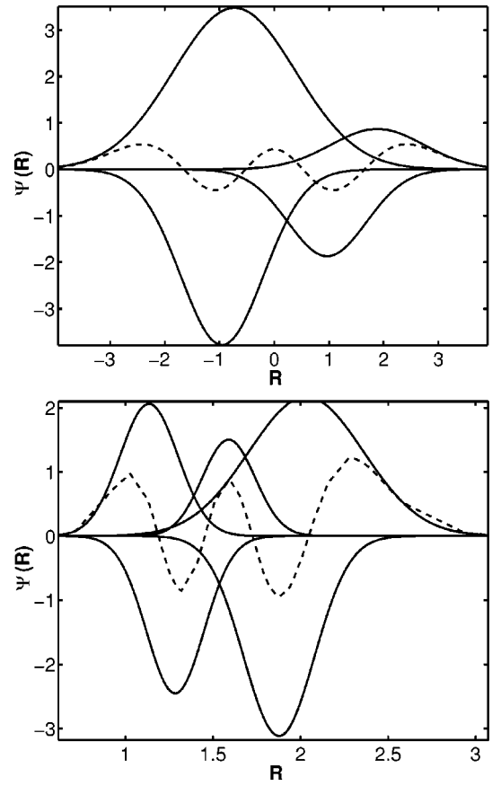
FIG. 2. Decomposition of v=4 bound state wave function (dashed) in terms of N Gaussian wave packets (solid). Upper: Harmonic oscillator with N=4 . Lower: Morse oscillator with N=5 .
