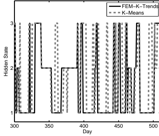
Figure 8: Comparison of transition paths calculated with K-means algorithm for \mathbf{K} = 3 (dashed) and FEM-K-trends algorithm for \mathbf{K} = 3, \mathcal{R} = 1, \epsilon^2 = 0 (solid).
