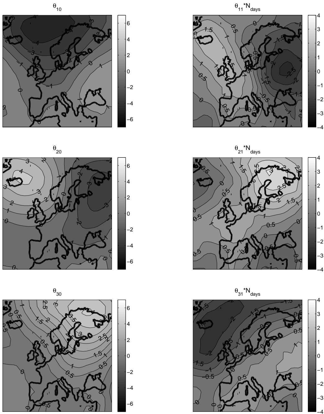
Figure 10: Regression coefficients (coloring in ^{\circ}\text{C} ) \theta_{i0}, i = 1, 2, 3 and the mean temperature change \theta_{i1} N_{\text{days}}, i = 1, 2, 3 resulting from FEM-K-trends clustering for K = 3, \mathcal{R} = 1, \epsilon^2 = 0 . Confidence intervals for the estimated parameters do not exceed 0.4^{\circ}\text{C} for \theta_{i0} and 0.2^{\circ}\text{C} for \theta_{i1}
