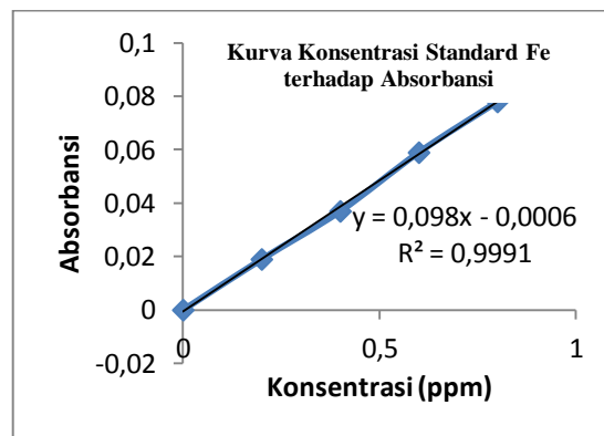
Gambar 2. Kurva kalibrasi larutan standar Fe(III)
