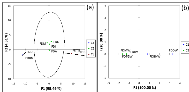
Figure 6 DA plots of (a) methanol extract of eight FD varieties and (b) water extract of five FD varieties
