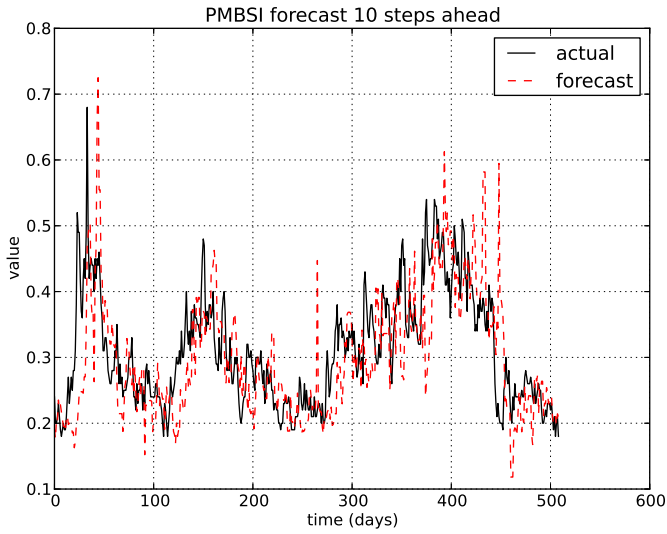
Figure 3. Forecast 10 steps ahead, PMBSI vs. the financial time-series
