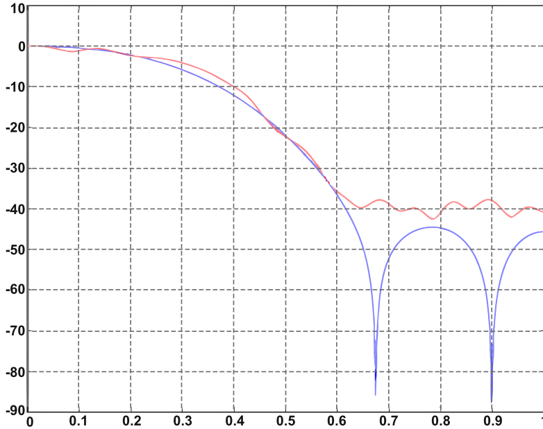
Fig. 6. Difference between filter in Matlab (blue) and on DSP processor (red)
