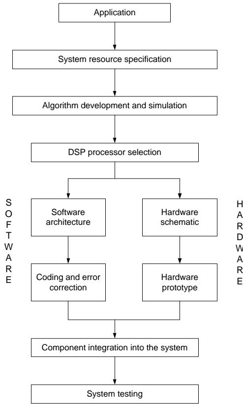
Fig. 3. Simplified diagram of a DSP system
