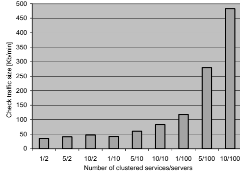
Fig. 13. Cumulative check-related network traffic generated on a LB computer with an active ATM
