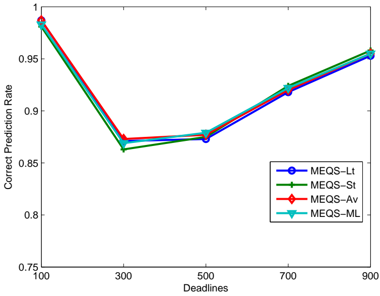
Fig. 11. Correct prediction rate of the MEQS predictor
