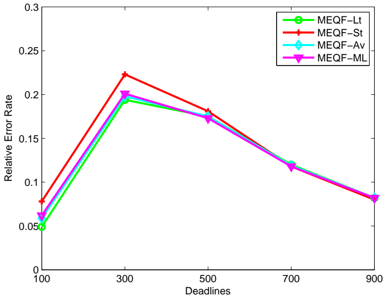
Fig. 8. Relative error rate of the MEQF predictor
