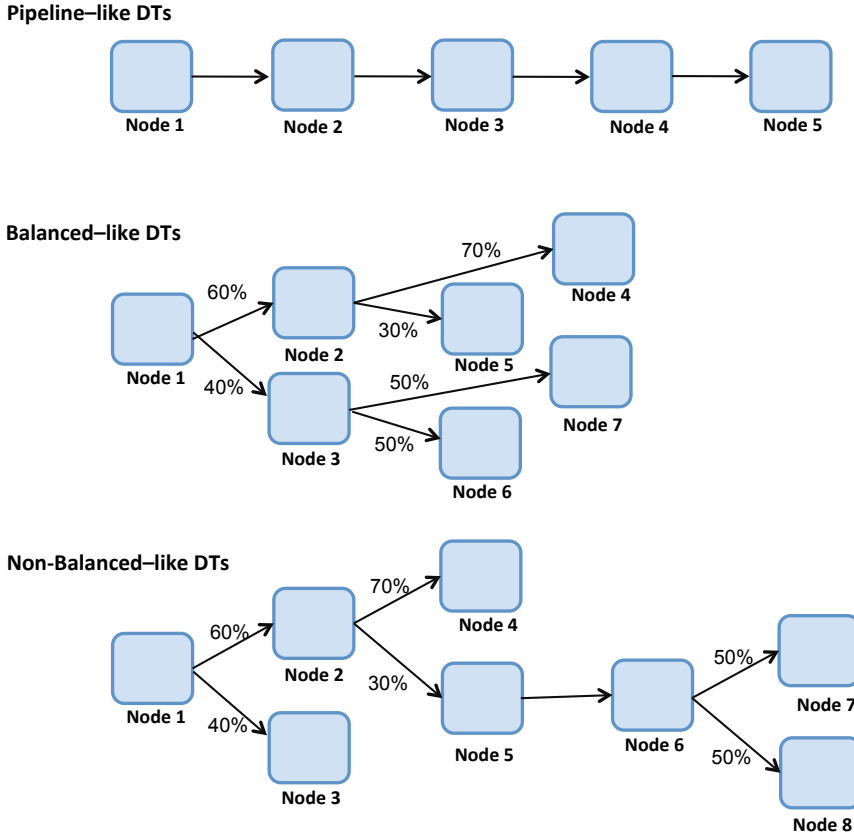
Fig. 5. Types of distributed threads
