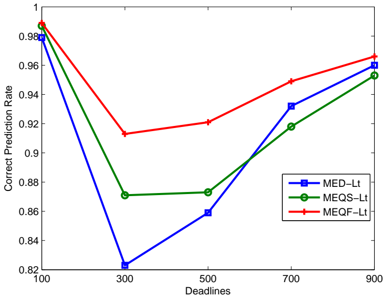
Fig. 13. Correct prediction rate of the MED, MEQS and MEQF mechanisms
