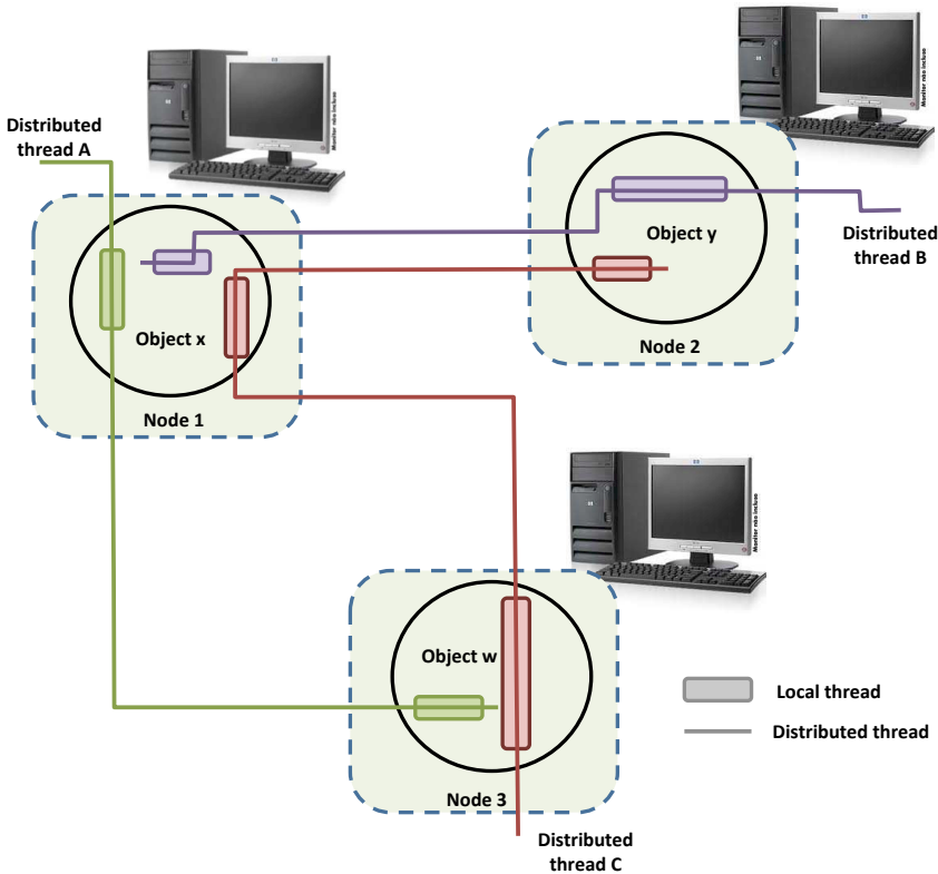
Fig. 1. Distributed threads and local segments
