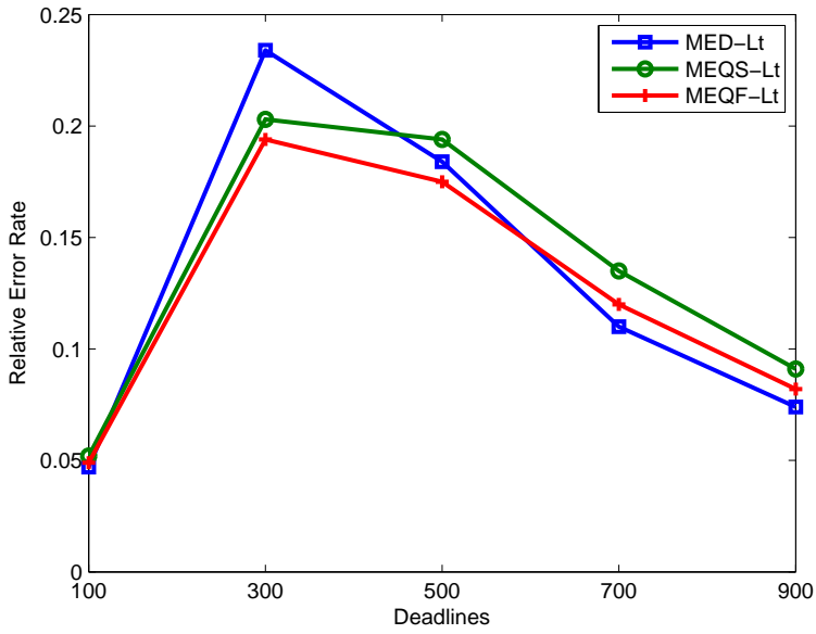
Fig. 9. Relative error rate of the MED, MEQS and MEQF mechanisms
