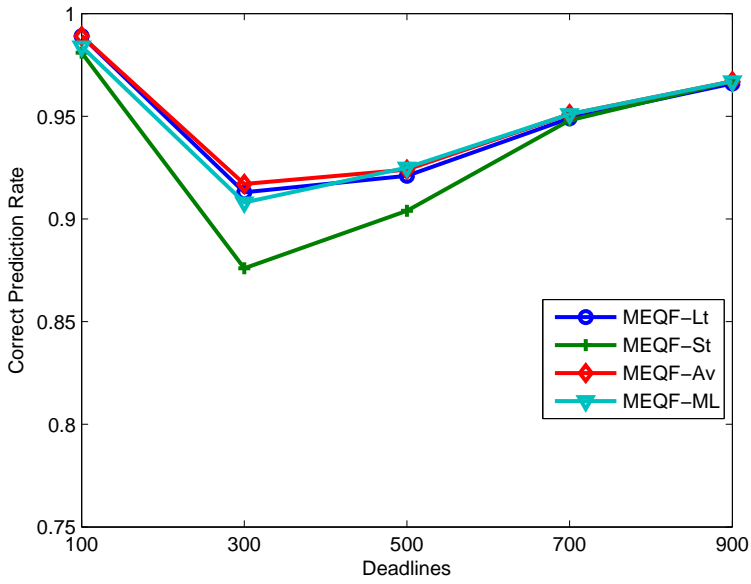
Fig. 12. Correct prediction rate of the MEQF predictor
