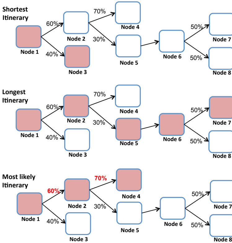
Fig. 4. Possible itineraries of a distributed thread
