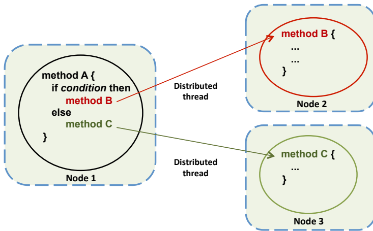
Fig. 3. Distributed thread execution flows alternatives
