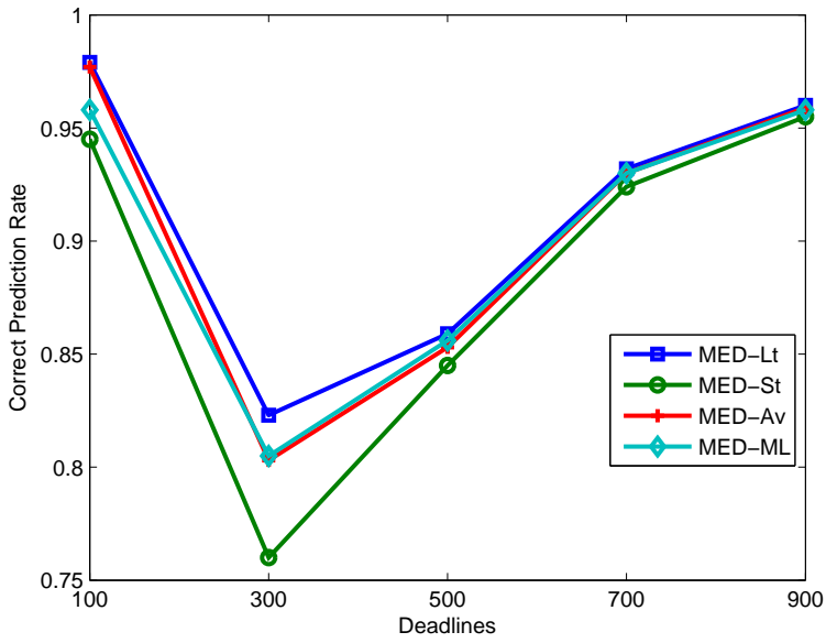
Fig. 10. Correct prediction rate of the MED predictor
