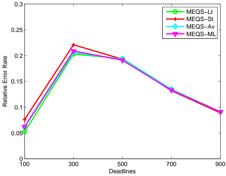
Fig. 7. Relative error rate of the MEQS predictor
