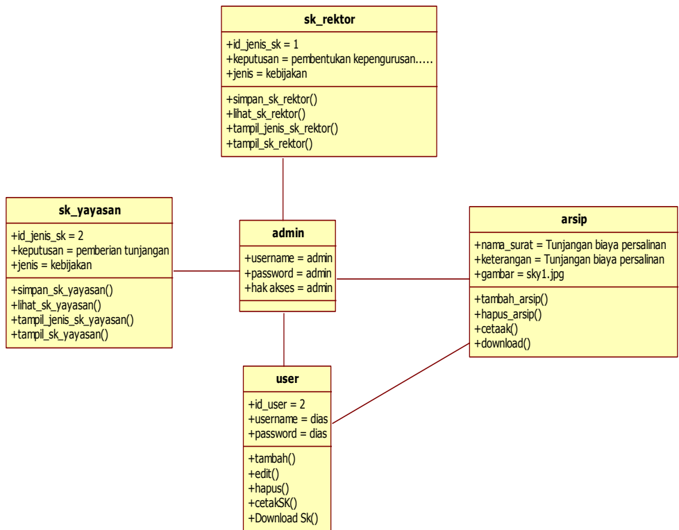
Gambar 4.3 Object Diagram
