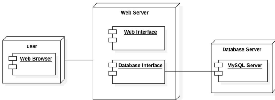
Gambar 4.4 Deployment Diagram
