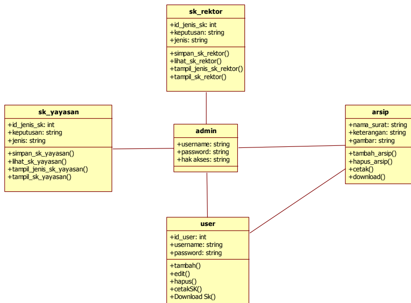
Gambar 4.2 Class Diagram
