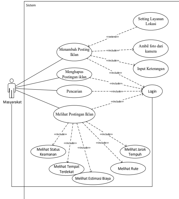
Gambar 10. Use Case Diagram
