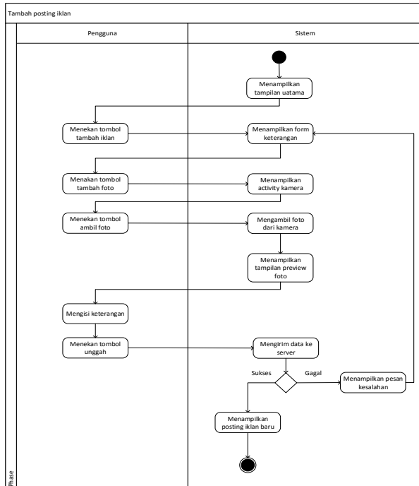
Gambar 11. Activity Diagram Tambah Posting Iklan
