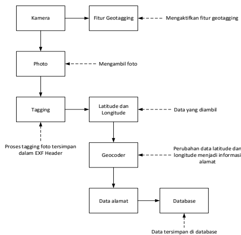
Gambar 6. Proses Pengambilan Data Geotagging
