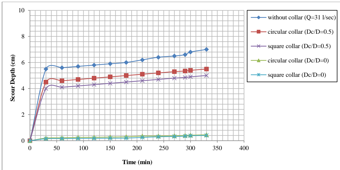
Figure 11. Scour depth of square collar of dimension 16×16 cm and circular collar of diameter 16 cm
