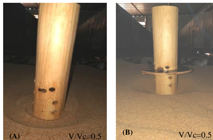
Figure 18. Scour depth of circular collar of diameter 16 cm collar on (A) bed level (B) collar above bed level
