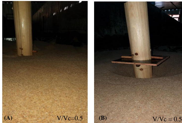
Figure 16. Scour depth of square collar of dimension 16×16 cm Collar on (A) bed level (B) collar above bed level
