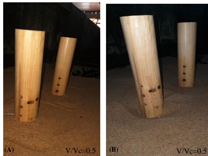
Figure 20. Scour depth of interaction of two piers; (A) square collar of dimension 24×24 cm on bed level; (B) triple collar of dimension 24×24 cm
