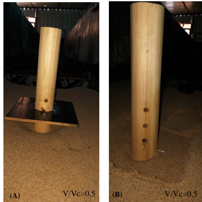
Figure 17. Scour depth of square collar of dimension 24×24 cm Collar on (A) bed level (B) collar above bed level
