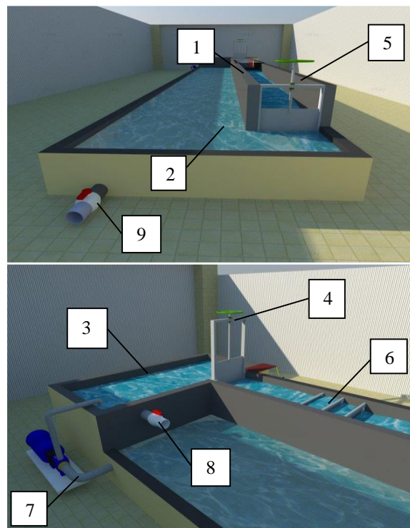
Figure 1. Laboratory channel: 1- The flume; 2- The lateral basin; 3- The head basin; 4- Vertical sluice head gate; 5- Vertical sluice tail gate; 6- Stilling screens; 7- Main pump; 8- Over flow pipe; 9- Lower flow pipe [24]
