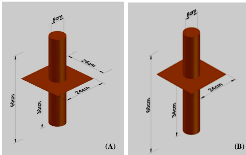
Figure 3. Square collar of dimensions 24×24 cm with two positions; (A) At bed level 30 cm (B) Above bed level 34 cm put in pier of diameter 8 cm and length 60 cm
