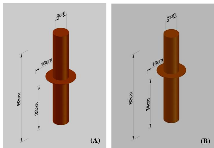
Figure 4. Circular collar of diameter 16 cm with two positions; (A) at bed level 30 cm (B) Above bed level 34 cm put in pier of diameter 8 cm and length 60 cm
