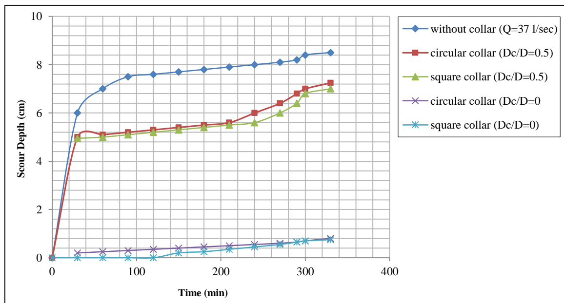
Figure 10. Scour depth of square collar of dimension 16×16 cm and circular collar of diameter 16 cm
