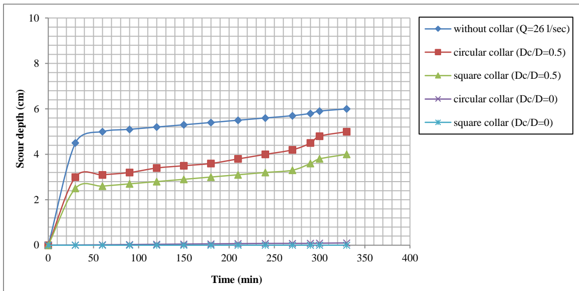
Figure 12. Scour depth of square collar of dimension 16×16 cm and circular collar of diameter 16 cm
