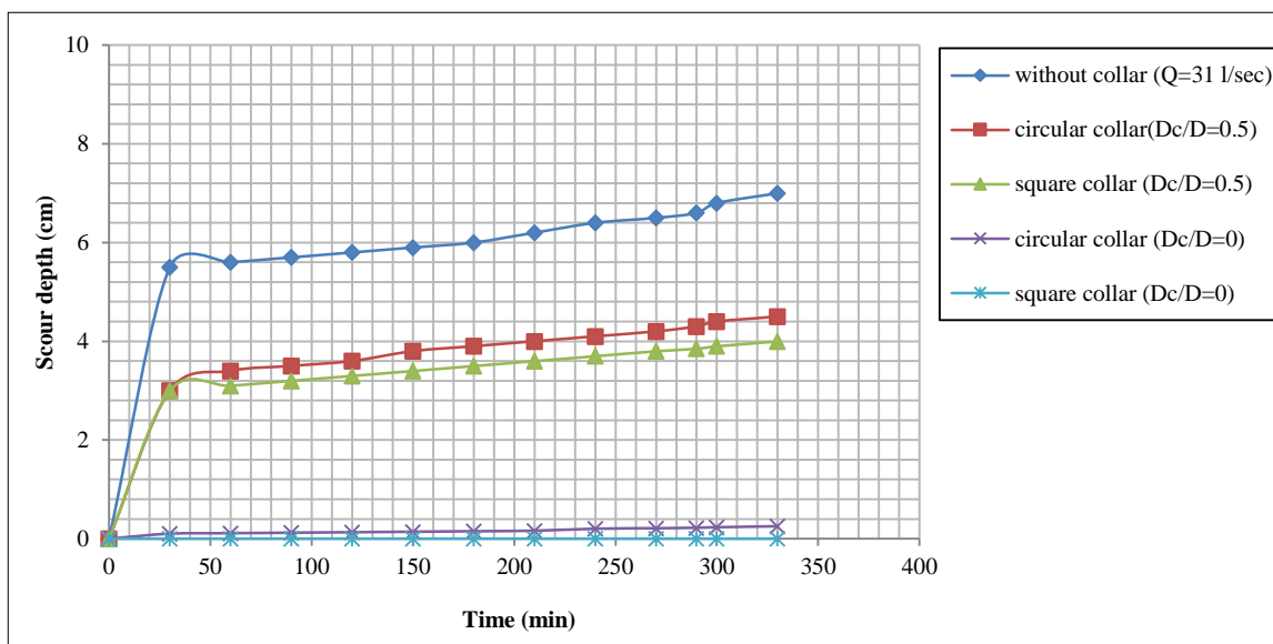
Figure 14. Scour depth of square collar of dimension 24×24 cm and circular collar of diameter 24 cm
