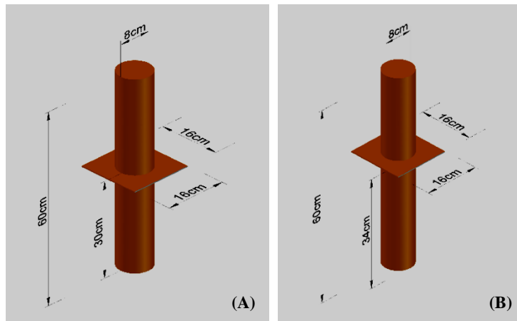
Figure 2. Square collar of dimensions 16×16 cm with two positions; (A) At bed level 30 cm, (B) Above bed level 34 cm put in pier of diameter 8 cm and length 60 cm
