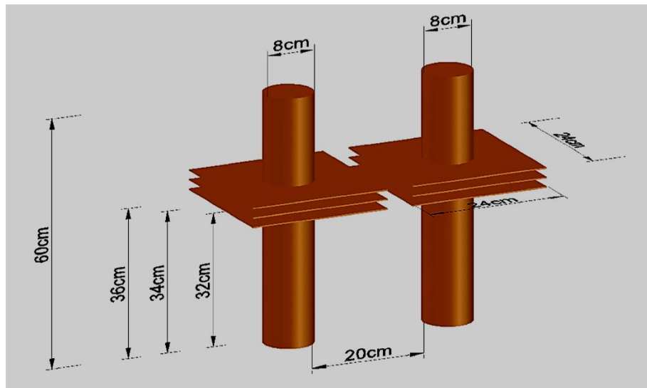
Figure 8. Interaction of two piers in a tandem arrangement with triple square collars of dimensions 24 \times 24 cm
