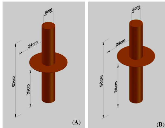
Figure 5. Circular collar of diameter 24 cm with two positions; (A) at bed level 30 cm (B) Above bed level 34 cm put in pier of diameter 8 cm and length 60 cm
