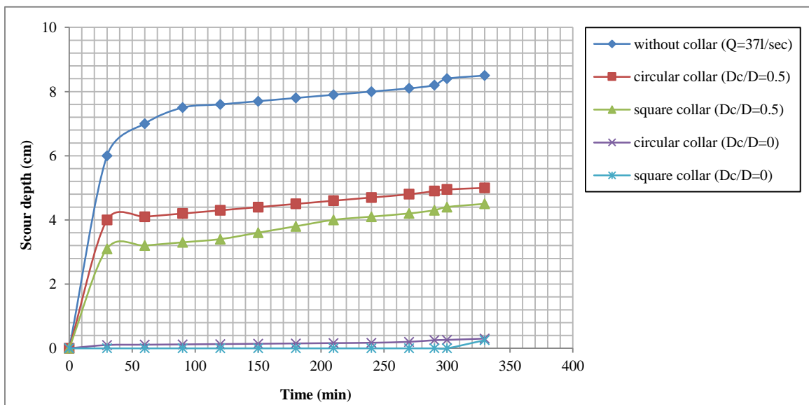
Figure 13. Scour depth of square collar of dimension 24×24 cm and circular collar of diameter 24 cm
