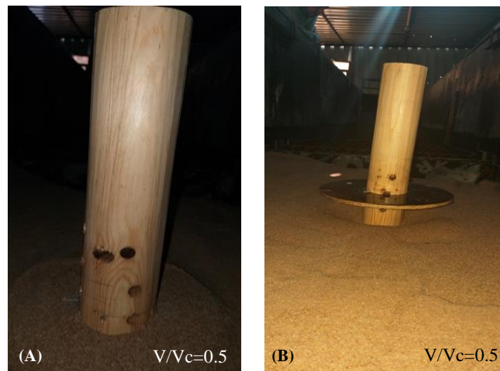
Figure 19. Scour depth of circular collar of diameter 24 cm collar on (A) bed level (B) collar above bed level
