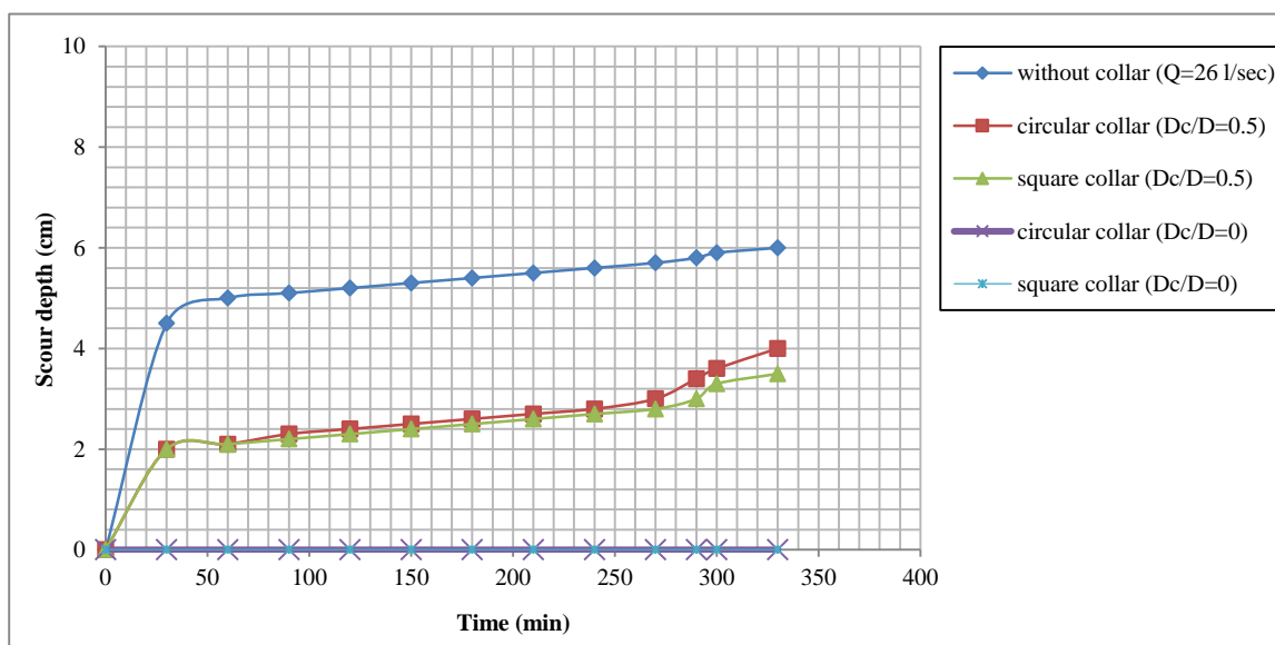
Figure 15. Scour depth of square collar of dimension 24×24 cm and circular collar of diameter 24 cm
