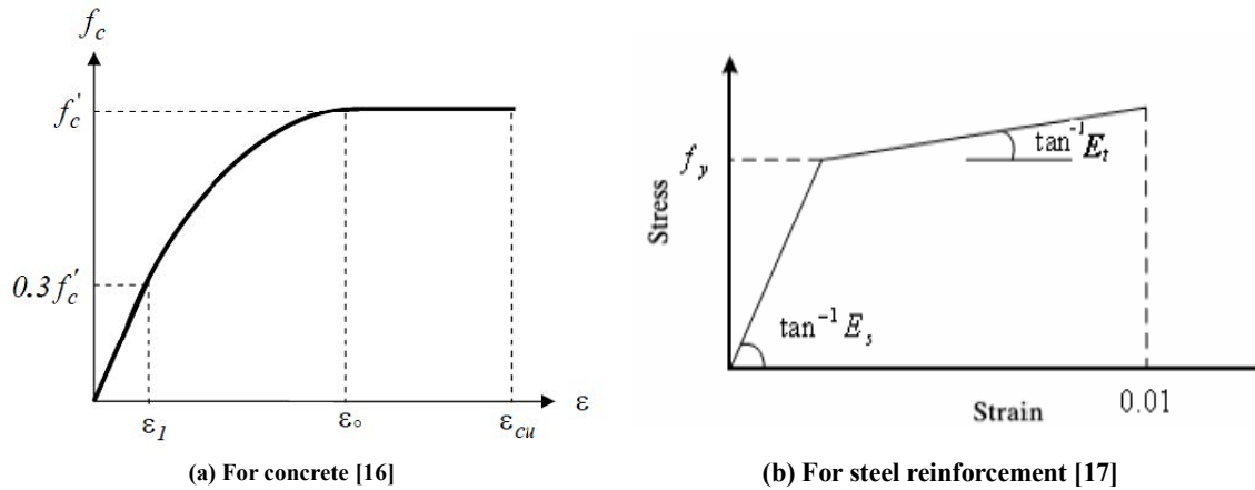
Figure 1. Stress- strain curve
